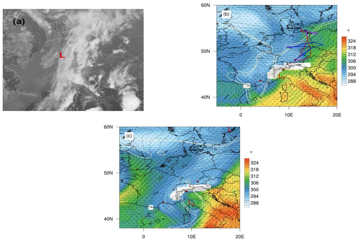
Figure 3. Continuation of the synoptic situation: (a) Meteosat IR image at 06 UTC 15 October 2012, (b) same as in Fig. 2a, but for 09 UTC 15 October and (c) 00 UTC 16 October 2012. In (b) flight IOP2b is shown in red with the violet part from 08:30 to 09:30 UTC, flight IOP2c in blue and the dark red 'L 2 ' marks the position of the secondary cyclone.
