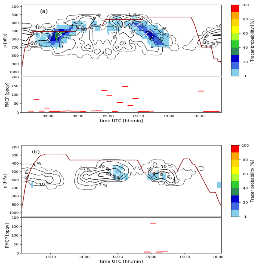
Figure 10. Tracer probability along the Falcon flights (a) IOP2b and (b) IOP2c. Upper panels show tracer probabilities (colours for all trajectories, white hatching for WCB trajectories), flight altitude (dark red line), WCB probabilities (black contours for 1, 10, 30, 60 and 90%), and the lower panels show the tracer concentrations sampled onboard the Falcon.
