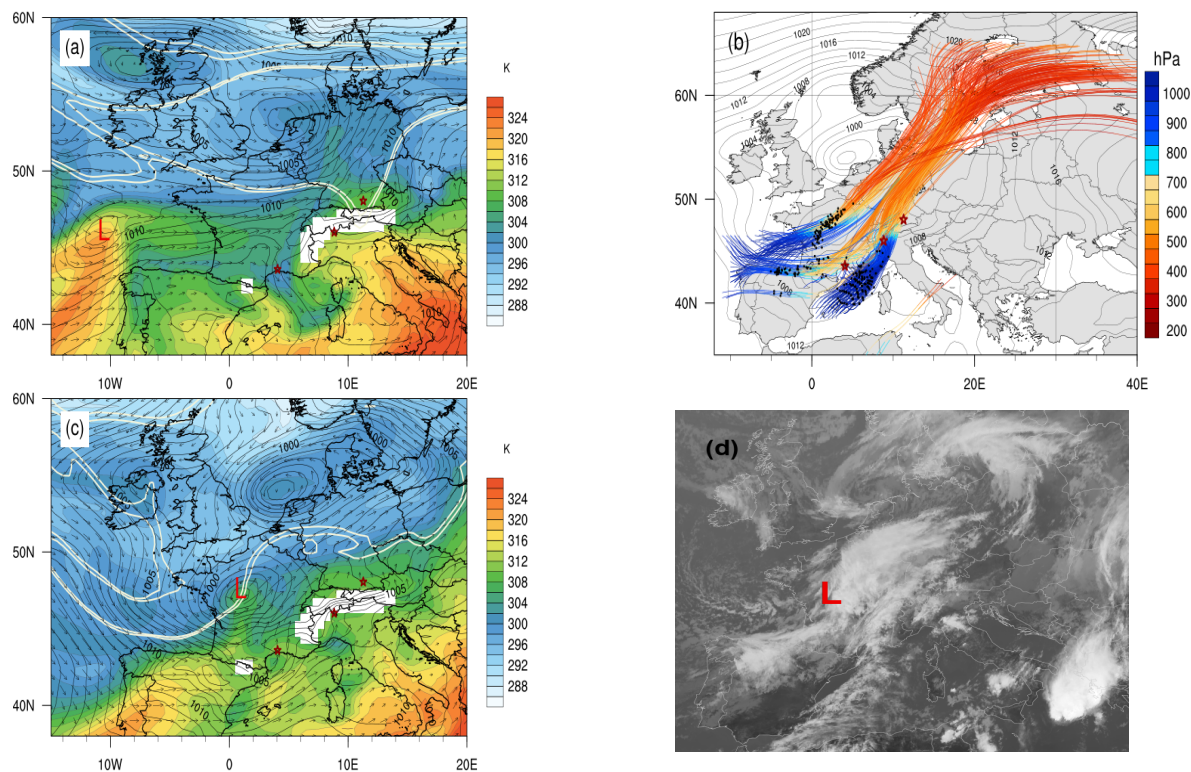
Figure 2. Synoptic development during the T-NAWDEx-Falcon IOP2: (a) EDA mean equivalent potential temperature at 850 hPa (colours, K), SLP (black contours every 1 hPa), wind arrows at 850 hPa (black) and PV at 315 K (white line of 1.5 and 2 pvu) at 18 UTC 13 October 2012. Red asterisks mark the measurement stations of the HyMeX lidar, Monte Lema radar and the air base of Falcon. (b) WCB trajectories of the EDA's CTL starting at 00 UTC 14 October 2012 (coloured by pressure, hPa) and SLP (black lines every 2hPa valid at 12 UTC 14 October), trajectory markers (black dots) for 12 UTC 14 October. (c) shows the same as (a) but for 12 UTC 14 October and (d) Meteosat infrared image at 12 UTC 14 October. The red 'L' in (a), (c) and (d) marks the location of the surface cyclone.
