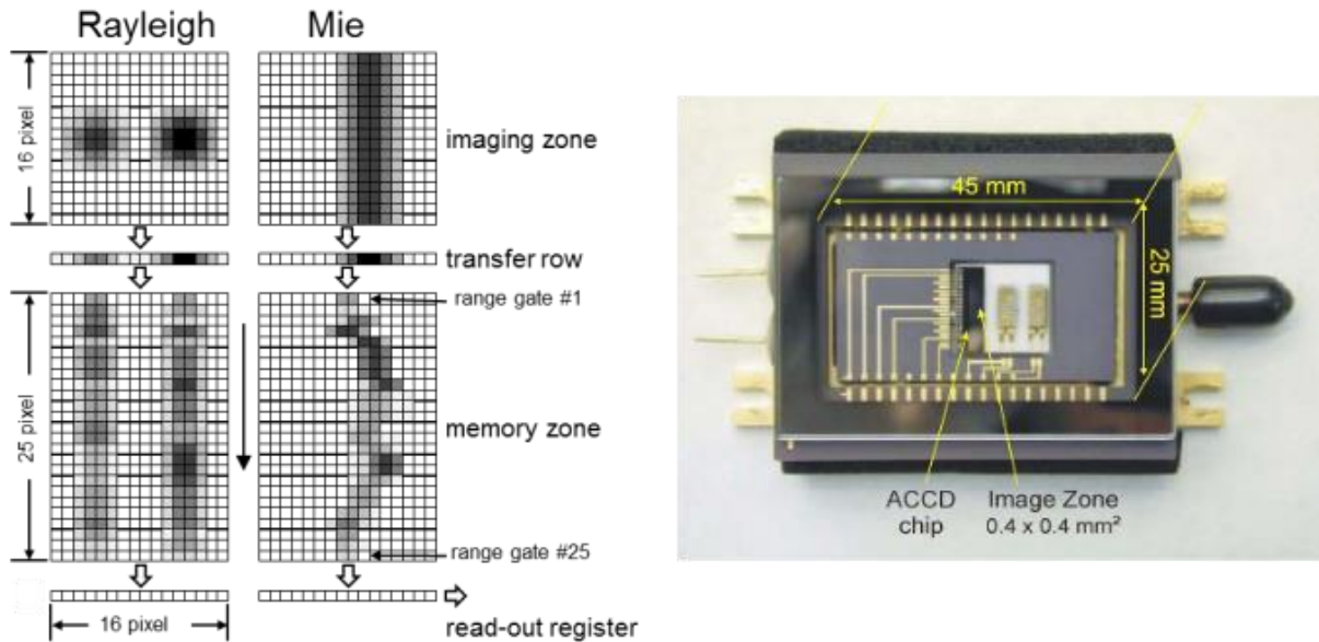
Figure 1: (left): Illustration of the Aeolus ACCDs with imaging zone, transfer row and memory zone for the Rayleigh and Mie channel (adapted from Marksteiner, 2013). (right): The detector with the ACCD chip housed in a thermo-controlled hermetically sealed package (ESA, 2008).
