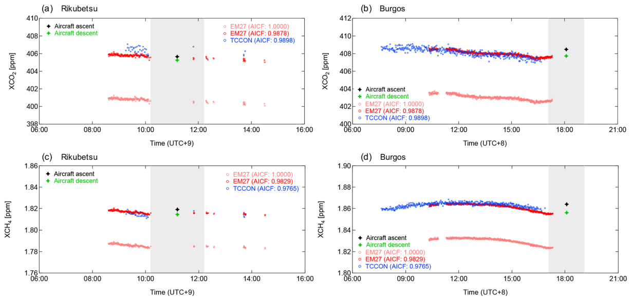
Figure 5. (a, b) XCO 2 and (c, d) XCH 4 values measured by the EM27/SUN, TCCON, and airborne instruments over (a, c) Rikubetsu on 27 April 2016 and (b, d) Burgos on 12 March 2018. The aircraft XCO 2 and XCH 4 values are calculated separately for the descending (green) and ascending (black) profiles shown in Figs. 1 and 3. Shown are the EM27/SUN values without air-mass-independent correction factors (AICFs = 1) and with them (AICFs \cong 1). The EM27/SUN data within the light gray shaded areas indicate \pm 1 h of the aircraft measurements and are used for determining the AICFs.
