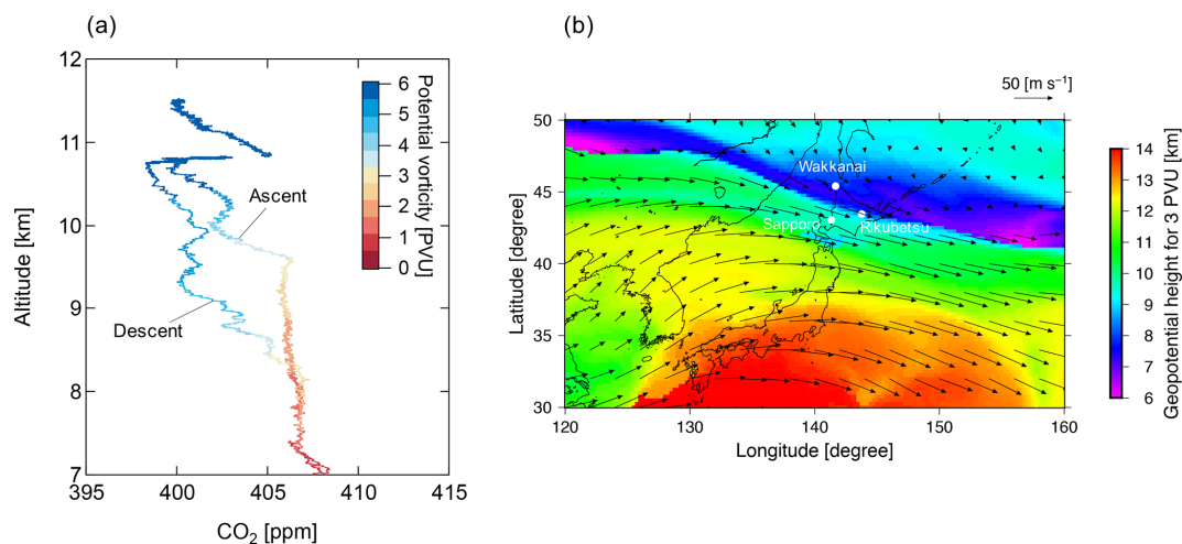
Figure 2. (a) The CO 2 profiles above 7 km over Rikubetsu. Colors denote the potential vorticity values from ERA5 (see text for details). (b) The ERA5 geopotential height (color scale) and winds (vectors) at the 3 PVU level on 27 April 2016, 02:00 UTC, are shown. White dots indicate the locations of Rikubetsu and two radiosonde stations in Hokkaido operated by the Japan Meteorological Agency (Sapporo and Wakkanai).
