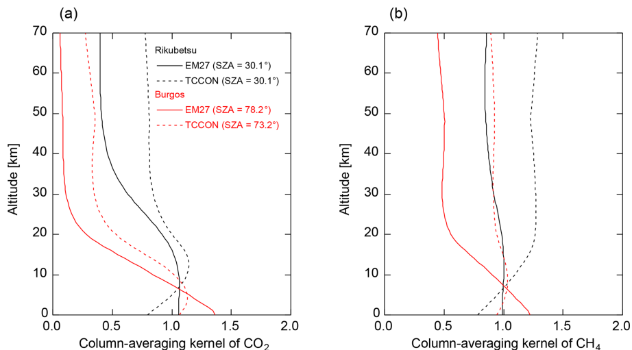
Figure 6. Column-averaging kernels of (a) CO 2 and (b) CH 4 retrievals from the EM27/SUN and TCCON spectra, which are used for calculating the aircraft XCO 2 and XCH 4 values over Rikubetsu (black) and Burgos (red).
