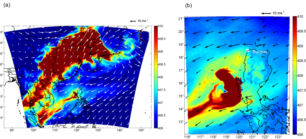
Figure 4. (a) Mean CO 2 mole fractions and wind vectors from the surface to 3 km altitude over Japan, Korea, China, Taiwan, and parts of Southeast Asia at 09:00 UTC on 12 March 2018, simulated by the Weather Research and Forecasting Model. (b) Same as (a) but for a magnified section over the Philippines at 10:00 UTC.
