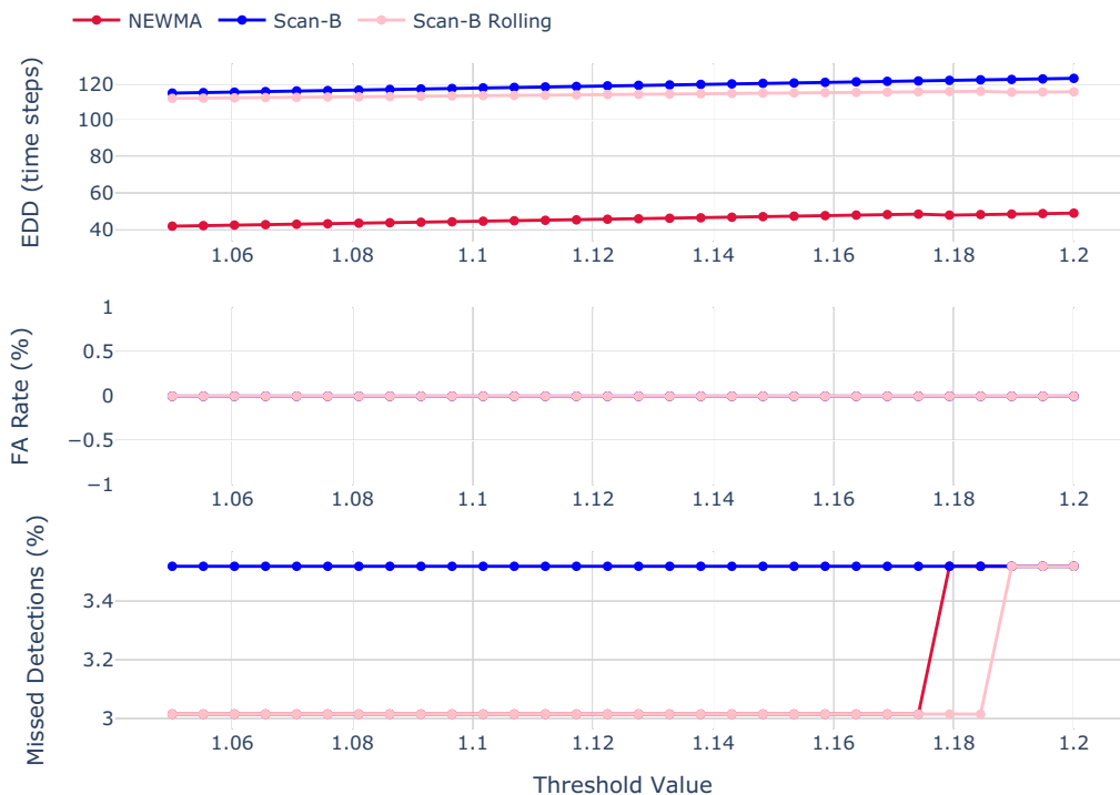
Figure 7: Evaluation graphs for a mean shift in a single dimension, where expected detection delay ( top ), false alarm rate ( middle ), and missed detection rate ( bottom ) are plotted over a threshold region between [1, 1.2].
