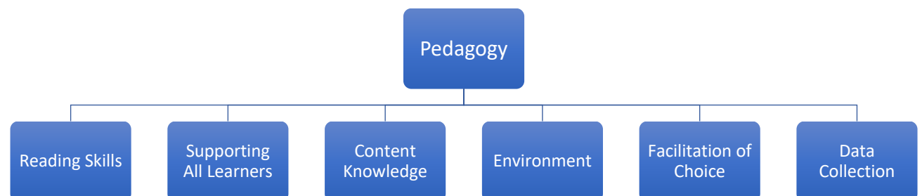
Figure 8. Pedagogy categories
