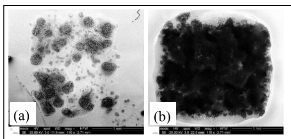
Figure 3. GO films at the silicon: one (a) and ten (b) depositions of 0.2- \mu l droplets.
