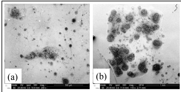
Figure 5. GO films on the Si surface: 1 W (a) and 4 W (b) of the applied power.
