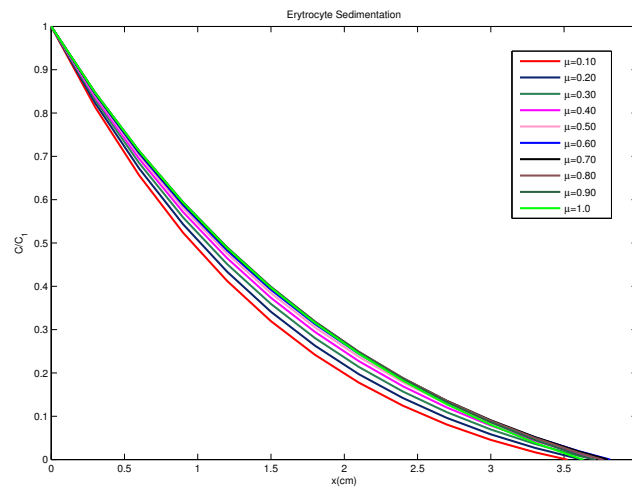
Figure 1. Analytic solution of fractional order PDE, Eq.(25).
