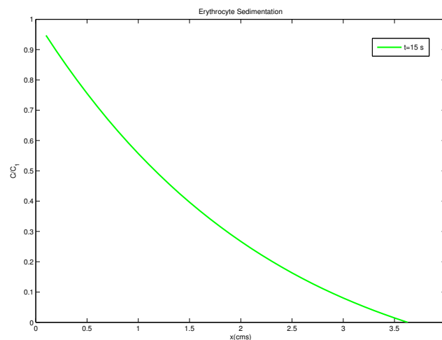
Figure 2. Analytic solution of integer order PDE.
