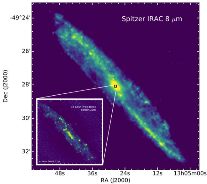
Figure 1. Spitzer IRAC 8 \mu\text{m} emission from UV-heated PAHs over the full galactic disk of NGC 4945. The black square indicates the 8'' \times 8'' ( 150 \text{ pc} \times 150 \text{ pc} ) central starburst region of interest in this paper; the inset shows the ALMA 93 GHz continuum emission.
