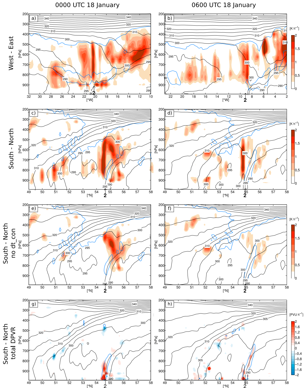
FIG. 5. West east and south north orientated vertical cross sections at (a),(c),(e),(g) 0000 UTC 18 Jan and (b),(d),(f),(h) 0600 UTC 18 Jan for 7 km grid spacing simulation. Positions of cross sections are marked in Fig. 4. (a),(b) West east cross sections depicting equivalent potential temperature \theta_e (K) in thin black lines (each 5 K), dynamical tropopause marked by 2 PVU line (bold blue line), and regions with diabatic heating rate ( \text{K h}^{-1} ) (shaded areas). (c),(d) As in (a),(b), but for south north cross sections. (e),(f) As in (c),(d), but for diabatic heating rate from cumulus parameterization excluded. Number “2” along the abscissa marks the corresponding cyclone positions of Kyrill II. (g),(h) Total DPVR ( \text{PVU h}^{-1} ) and the z component of absolute vorticity \eta_p ( \text{blue line at } 0.5 \times 10^{-4} \text{ s}^{-1} ).
