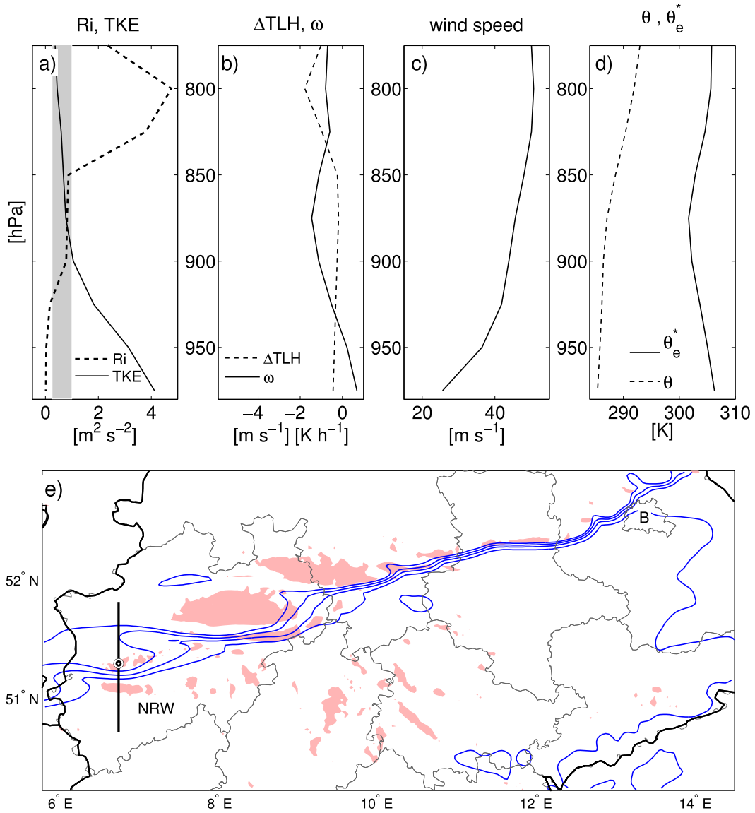
FIG. 9. Vertical profiles at 51.28°N, 6.76°E and at 1645 UTC 18 Jan. (a) Gradient Richardson number [Ri, dimensionless: shaded area (gray) marks the transition between stable ( Ri > 1 ) and turbulent flow ( Ri < 0.25 )] and turbulent kinetic energy [TKE ( \text{m}^2 \text{s}^{-2} )]. (b) Vertical velocity [ \omega ( \text{m s}^{-1} )] and diabatic heating rate [ \Delta\text{TLH} ( \text{K h}^{-1} )]. (c) Magnitude of horizontal wind speed ( \text{m s}^{-1} ). (d) Potential and equivalent potential temperature of saturated air [ \theta, \theta_e^* (K)]. (e) Areas over central Germany [including federal state borders; North Rhine Westphalia (NRW); Berlin (B)] with instantaneous gust wind speed at 1645 UTC exceeding 32.7 \text{ m s}^{-1} marked in red. Equivalent potential temperature ( \theta_e ) along the front region at 950 hPa marked with blue contours (lines between 300 and 306 K with interval of 2 K) with higher values to the south. Black/white circles mark the locations of vertical profiles. The front normal cross section depicted in Fig. 11a is marked by a bold black line.
