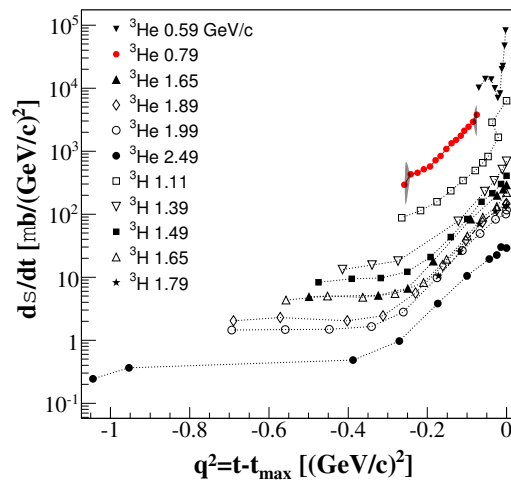
Figure 4: (Color online) Differential cross sections for transfer reactions in d - d scattering q^2 [29, 30]. The data from the BINA experiment at 0.79 GeV/c are shown as red points. The dark band represents systematic errors. For more details see Ref. [33].
