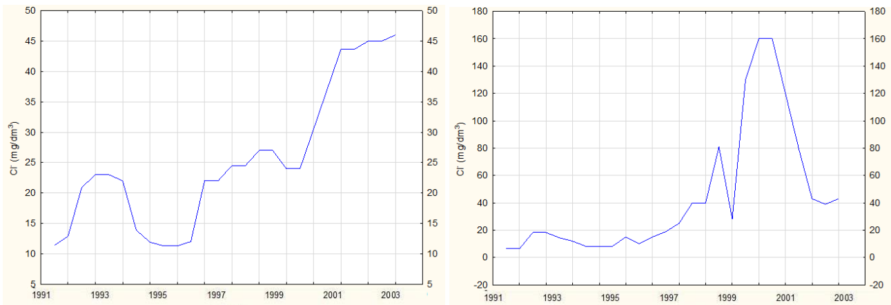
Fig. 4. Changes in chloride content in piezometers T1 and Q1 obtained with the moving median method
