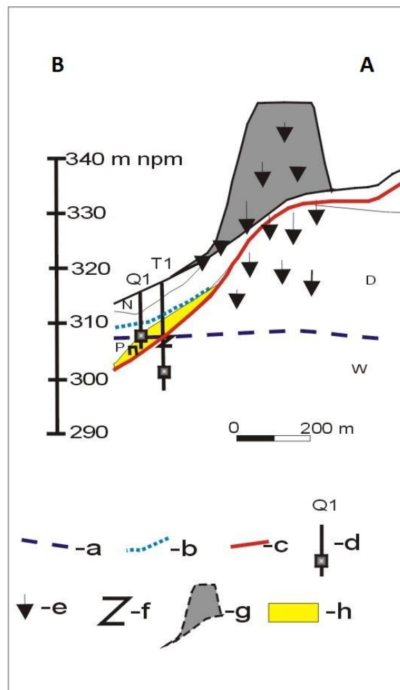
Fig. 2. Hydrogeological cross section N-S through the area of the metallurgical Lipówka landfill site (a) groundwater table in the Triassic sediments; (b) groundwater table in the Quaternary sediments; (c) stratigraphic boundary; (d) piezometer; (e) direction of seepage from the landfill; (f) confined table; (g) the Lipówka landfill; (h) poorly permeable Quaternary sediments; (w) limestone; (D) dolomites; (P) sands, (II) dust; (N) embankment
