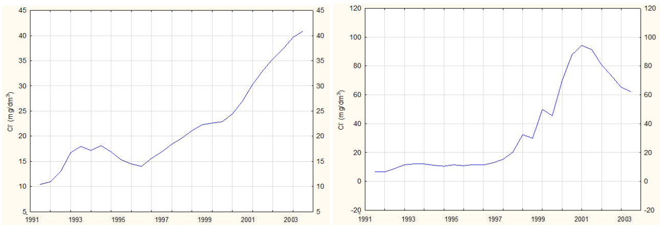
Fig. 5. Changes in chloride content in piezometers T1 and Q1 obtained with the exponential smoothing method
