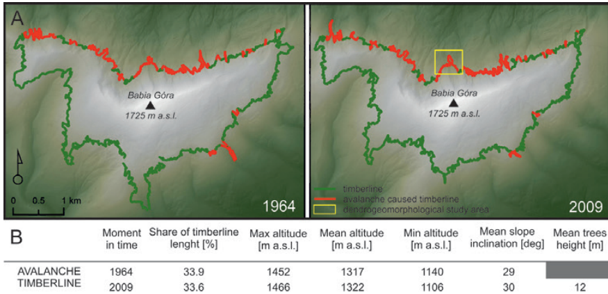
Figure 4. The timberline on the Babia Góra massif modified by the avalanches of 1964 and 2009. Spatial distribution of the TEa (A) and its basic parameters (B)
