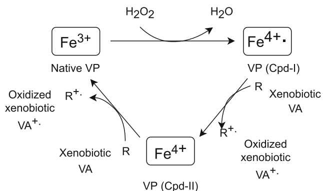
Fig. 5 VP catalytic cycle during oxidation of VA and nonphenolic compounds (Abdel-Hamid et al. 2013, modified)
