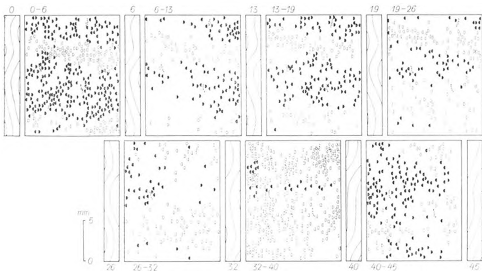
Fig. 7. Fraxinus excelsior , sample 2. Events occurring during the formation of the annual rings No. 50—56. Legend as in Fig. 6.
