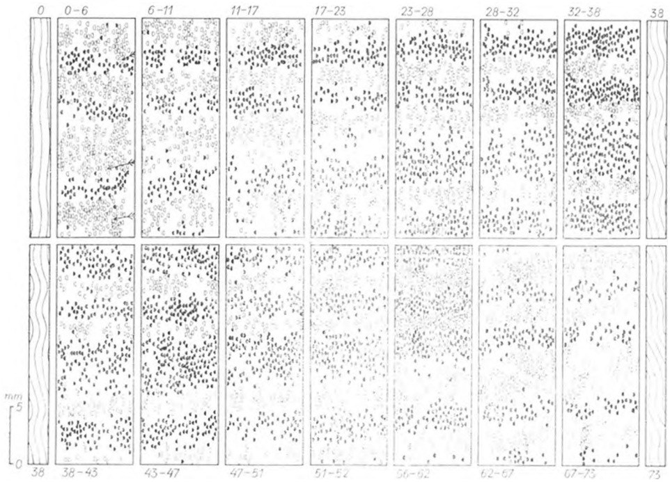
Fig. 6 Fraxinus excelsior , sample 1. Wide rectangles with semicircles denote ray splitting and uniting, respectively. Full symbols denote S events, empty symbols Z events. Some rays used as position indices are shown, indicated by arrows on the 1st map. The successive maps are displaced slightly transversely to the right but are not displaced longitudinally, thus upward displacement of the domains represents the migration of the domain pattern. Pulsation of the domains in length may be seen. The figures show the position, in mm., of the annual rings with respect to the inner border of the 19th ring (from the pith). The narrow maps show the course of grain at the indicated positions (0, 38, 73 mm).
