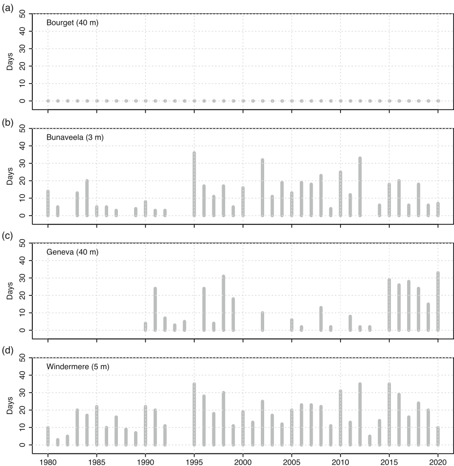
Fig. 4 Longest consecutive number of days during each November and December spawning season, where the maximum daily temperature exceeded 8.5 °C 1980–2020 for a Lake Bourget at 40-m depth, b Lough Bunaveela at 3-m depth, c Lake Geneva at 40 m, and d Windermere at 5 m
