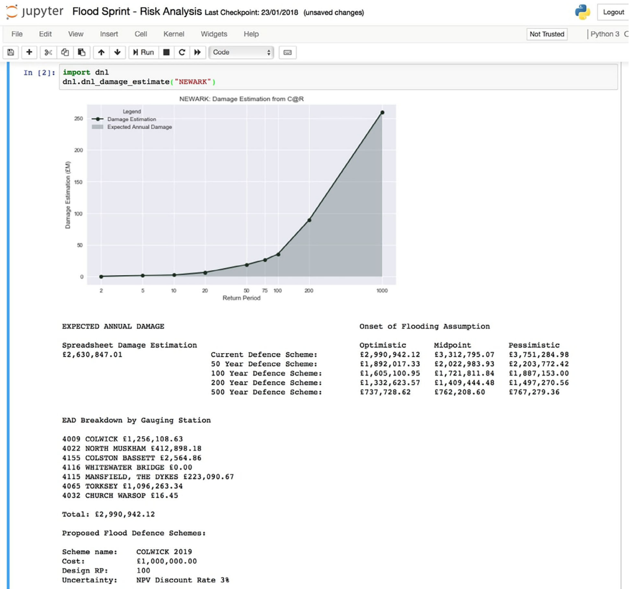
FIGURE 9 Estimated expected annual damages with associated metadata for Newark-on-Trent from the flood risk demonstrator. The expected annual damage has been broken down by gauging stations with information also provided on proposed flood defence schemes
