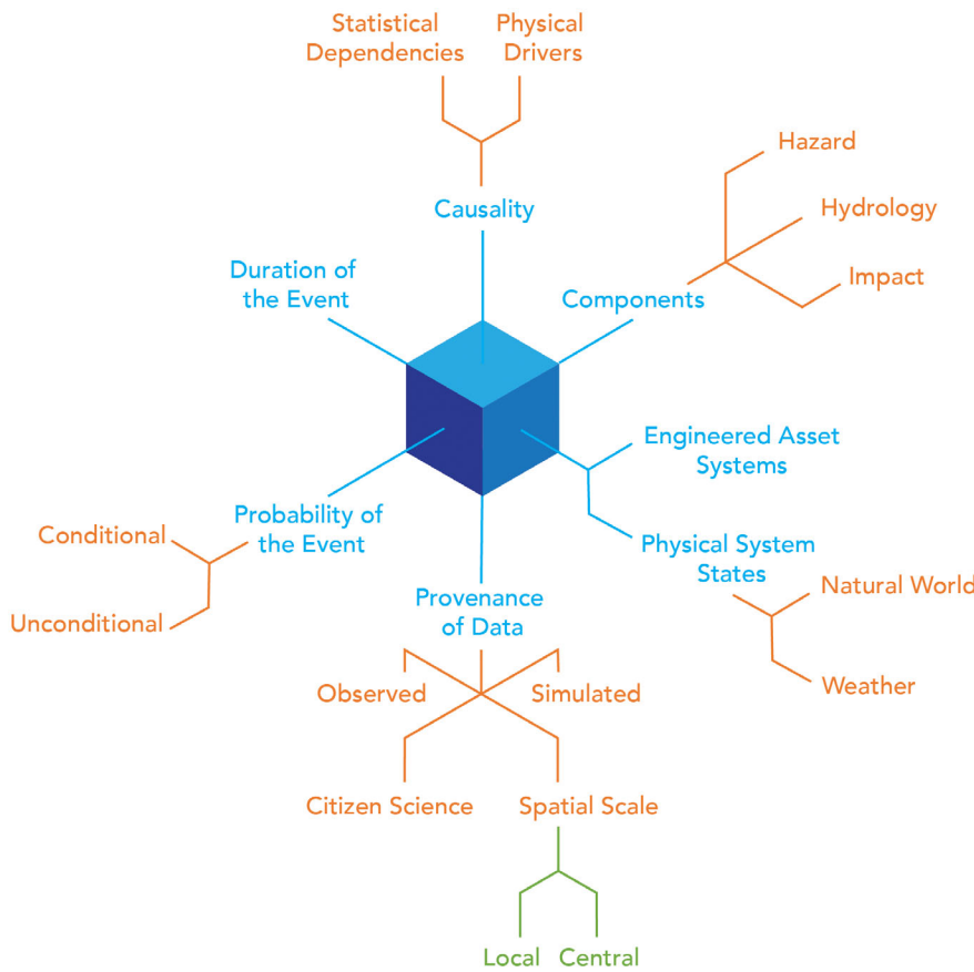
FIGURE 3 The concept of a data hypercube for a flood event
