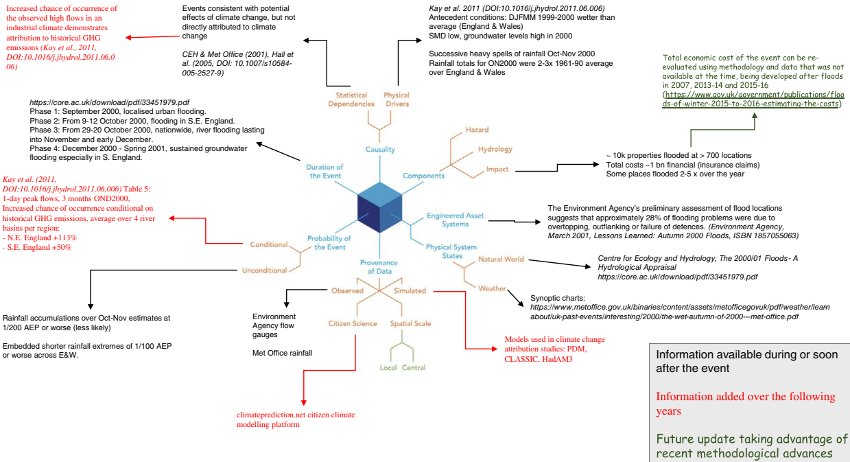
FIGURE 4 An instance of the data hypercube populated with information about a specific flood event, in this case the flooding that happened in the Autumn and Winter of 2000 in the United Kingdom
