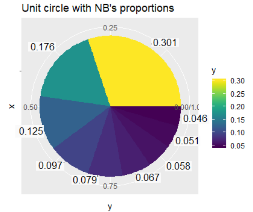
Figure 4.1. Pie chart of the unit circle with the different probabilities of NBL.
