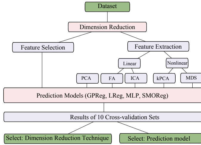
Fig. 1. Experimental setup for the identification of the dimensionality reduction and selection prediction model for the prediction of PLGA dissolution profile.
