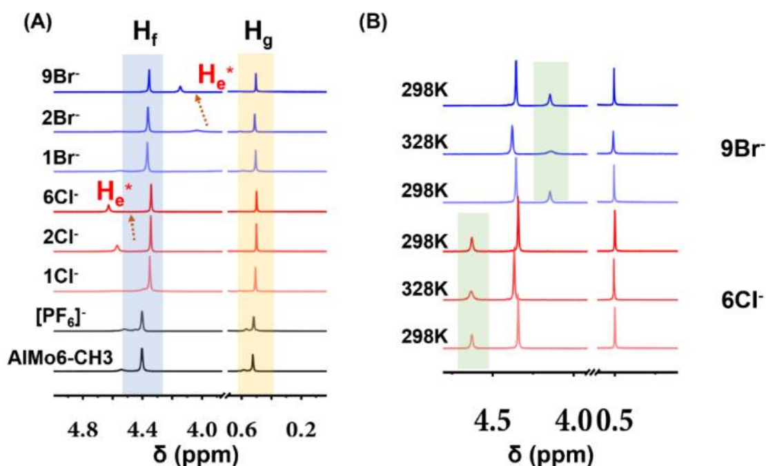
Figure 3. a) Investigation on halide ion adding into \text{AlMo}_6\text{CH}_3 at 10.0 mM in acetonitrile- d_3 at 298K; b) Variable temperature ^1\text{H} NMR spectrum to detect the hydrogen bond between POM and halide ion.
