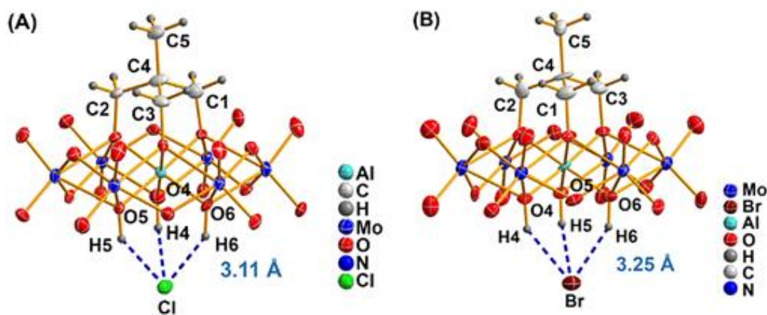
Figure 1. Molecular structures of a) AlMo_6CH_3 \cdot Cl b) AlMo_6CH_3 \cdot Br , with thermal ellipsoids are drawn at the 50% probability level.
