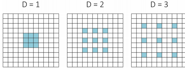
Figure 1. Atrous convolutions allow the network to obtain varying spatial resolution by changing the dilation rate ( D ). The number of parameters to learn (in this figure, 9, one for each coloured square) does not change, since the empty elements within the filter are filled with zeros. (Image from (91))
