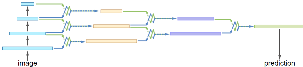
Figure 2. Architecture of the MSCI network. On the left, a traditional convolutional neural network encodes features into layers of progressively smaller reception fields. Each pair of adjacent layers is connected “horizontally” using bi-directional connections, which progressively incorporate information from different receptive fields into the final prediction (to the right). (Image courtesy of (98))
