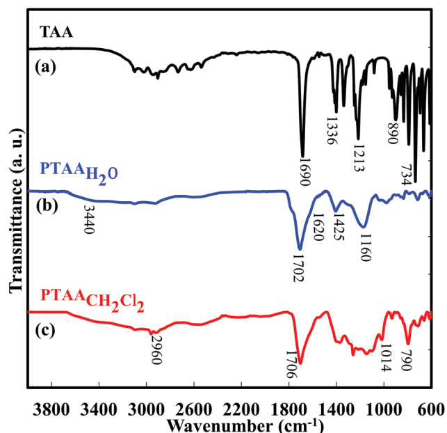
Fig. 3 ATR-FTIR spectra of (a) pure TAA monomers, (b) PTAA H 2 O and (c) PTAA CH 2 Cl 2 . The polymers were synthesized by \gamma -induced polymerization in water under N 2 O or in DCM under N 2 at irradiation doses of 38 kGy and 36 kGy respectively. The initial concentration was 10 mM TAA.
