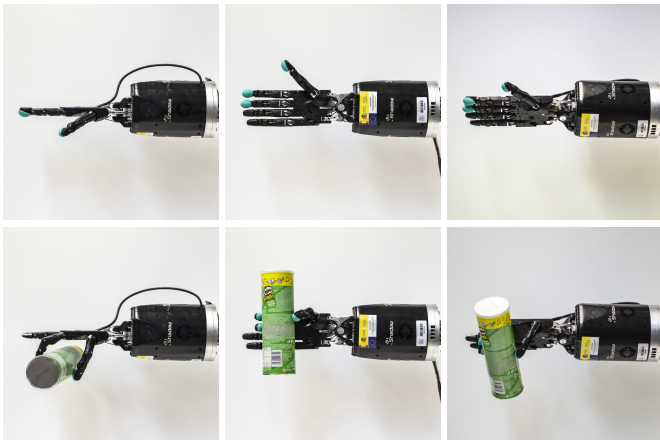
Fig. 7: (Top row) Samples of the three hand configurations in the dataset: (from left to right) palm down , palm side , and palm 45 . (Bottom row) The same configurations but grasping an object.
