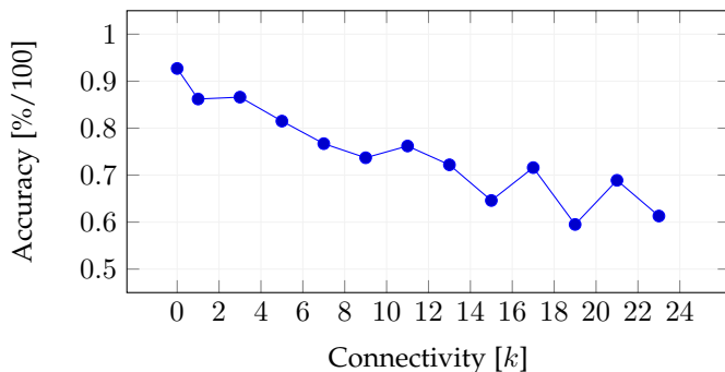
Fig. 9: Performance of the network according to the connectivity of the graph.
