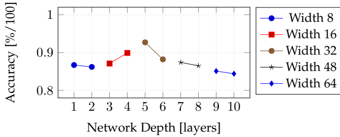
Fig. 8: Results of network depth and width study.
