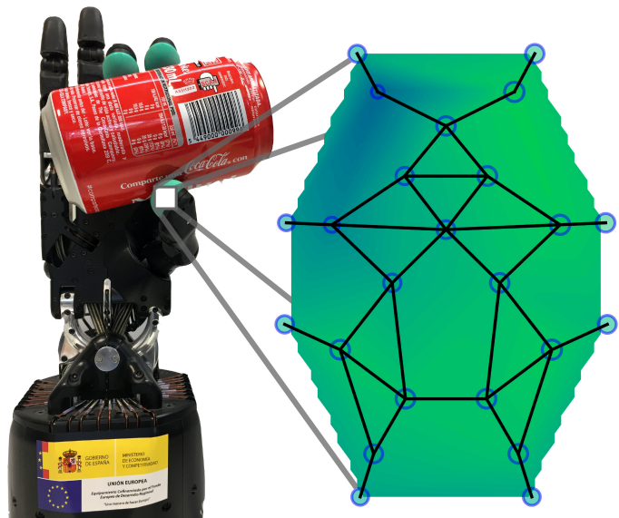
Fig. 1: In this work, we use a Shadow Dexterous hand equipped with three BioTac SP tactile sensors whose readings are transformed into graph representations. Those graphs are then fed as input to a GNN to learn to predict grasp stability.
