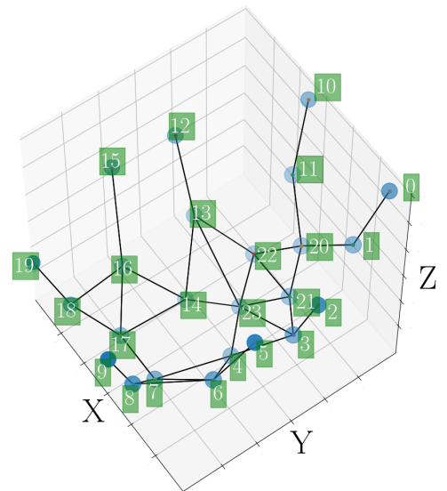
Fig. 3: 3D visualization of the tactile graph layout using the accurate spatial arrangement from the actual BioTacSp sensor. Graph edges correspond to the manually defined connections.
