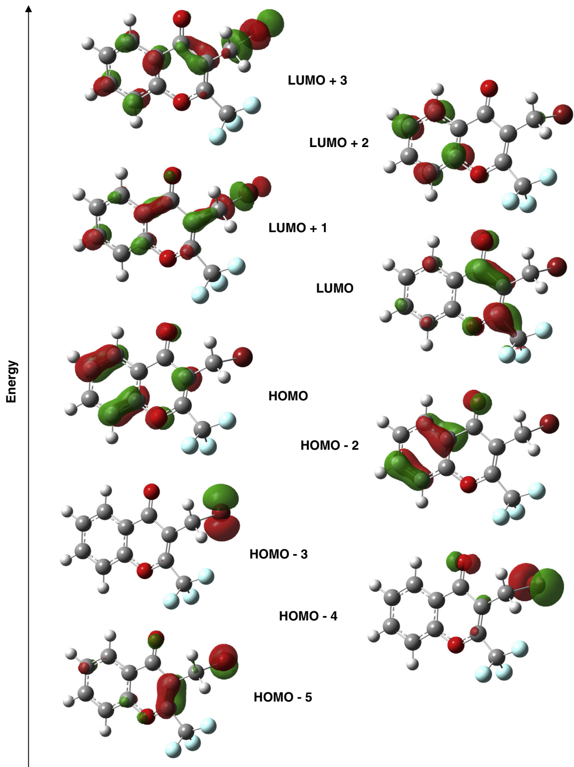
Fig. 11. Molecular orbitals involved in the electronic transitions of 3-bromomethyl-2-trifluoromethylchromone ( 2 ). The energy scale is only qualitative and does not represent the actual energy of the molecular orbitals.
