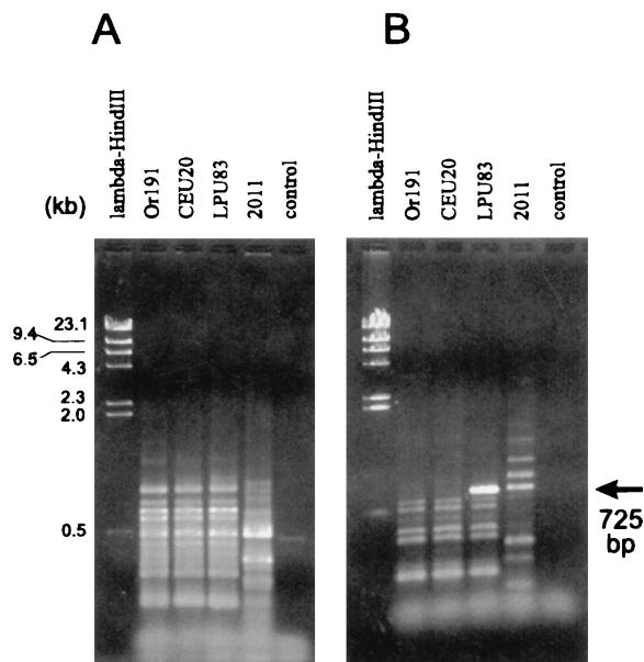
FIG. 4. MBOREP1 and BOXC1 PCR-fingerprinting patterns of representative AT isolates from central Argentina and Uruguay. Panels A and B show the patterns of PCR products generated by using chromosomal DNA of the indicated strains and primer MBOREP1 or BOXC1, respectively. The DNA molecular-weight standard corresponding to restriction fragments of the lambda phage digested with Hind III is indicated on the left side of each panel. The arrow on the right side designates the differential BOXC1 amplicon of ca. 725 bp, which was only detected in the AT isolate LPU83. Agarose gels containing ethidium bromide were photographed with Polaroid type 667 film under UV illumination. Pictures were scanned with a Hewlett-Packard ScanJet4C (high resolution), composed with Corel Draw 5, and printed with a Rainbow-3M dye sublimation primer.
