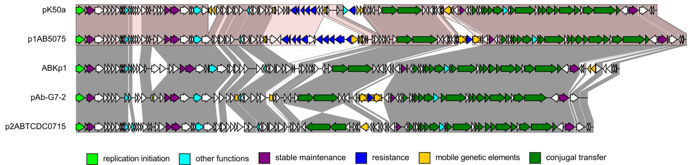
FIG 5 Comparative analysis of five A. baumannii plasmid genome sequences. Homologous gene clusters between plasmids pK50a, p1AB5075, ABKp1, pAb-G7-2, and p2ABTCD0715 were computed by means of M-GCAT (69) and are displayed as regions highlighted in gray. Homologous gene clusters of plasmids pK50a and p1AB5075 are highlighted in light red. Annotated coding sequences are displayed as arrows, and repetitive elements are displayed as rectangles. Coding sequences are colored based on their assigned gene functions.
