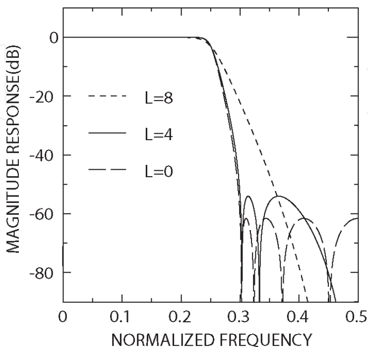
Figure 6. Magnitude responses of H_0(z) in example 2.
