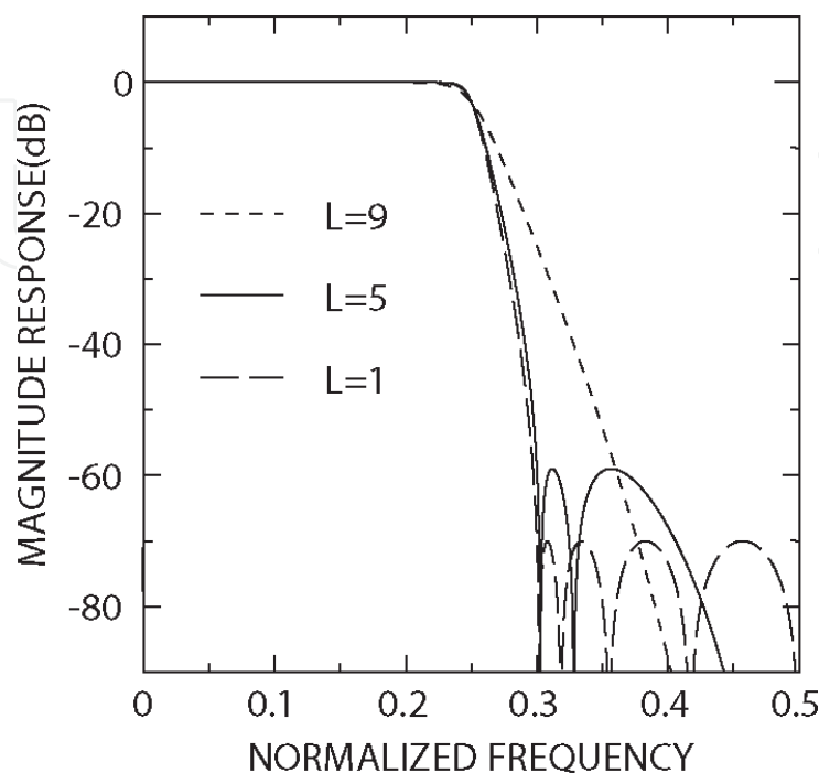
Figure 3. Magnitude responses of H_0(z) in example 1.
