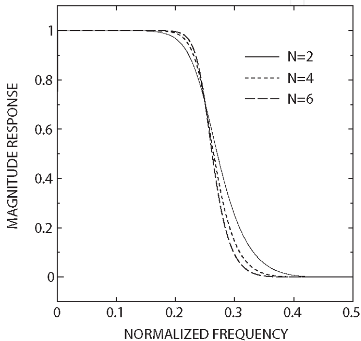
Figure 15. Magnitude responses of H_0(z) in example 6.
