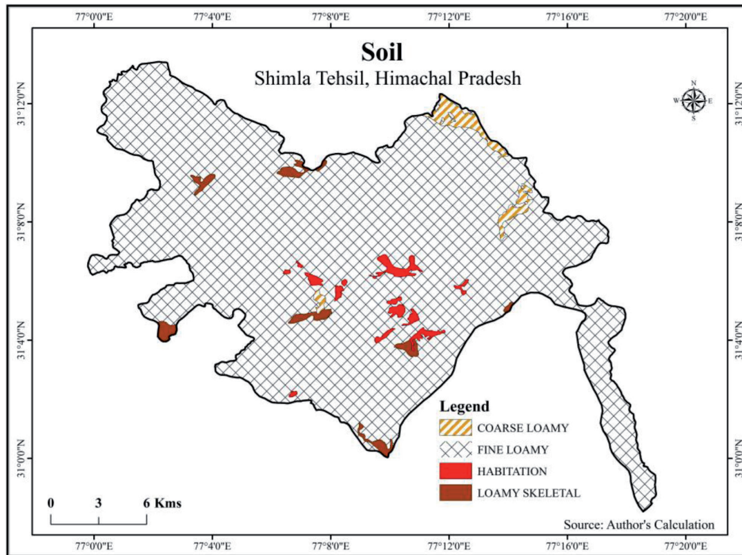
Figure 5. Soil.
