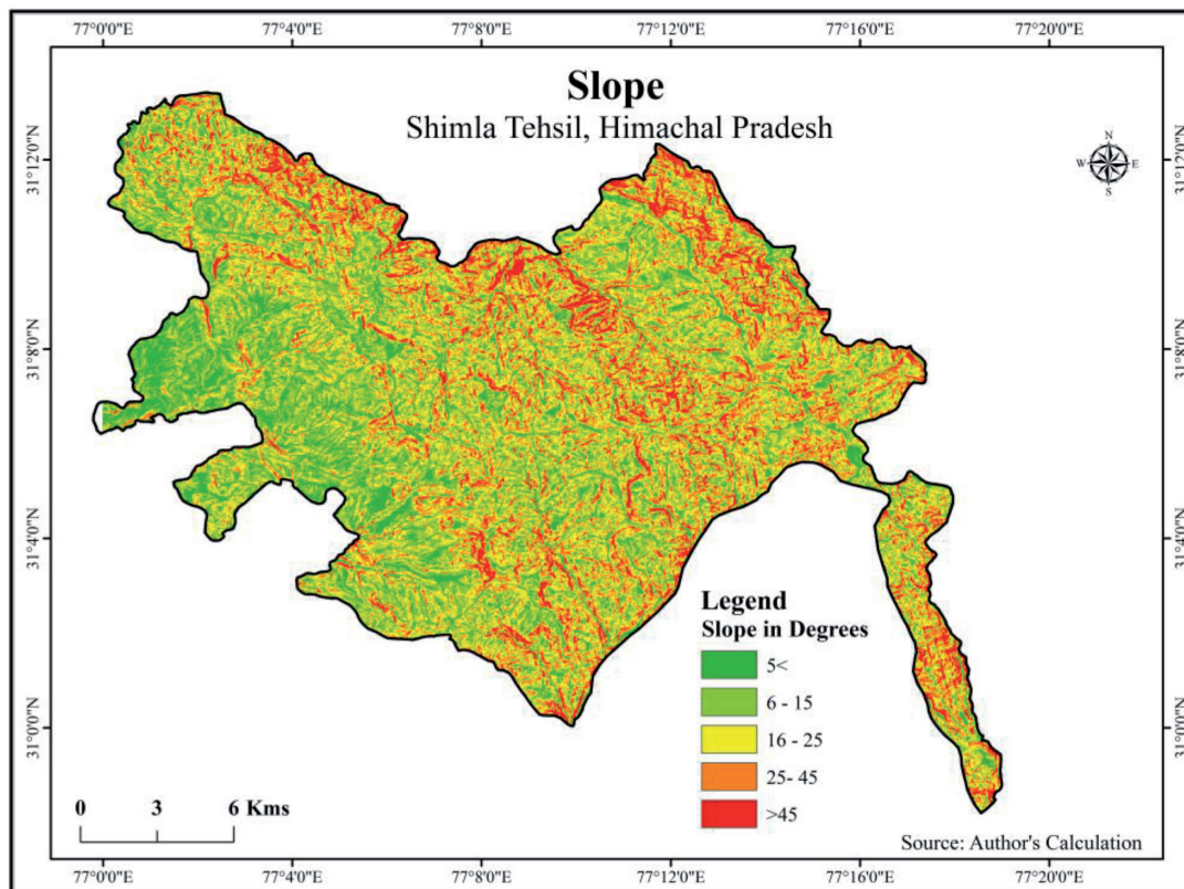
Figure 9. Slope.
