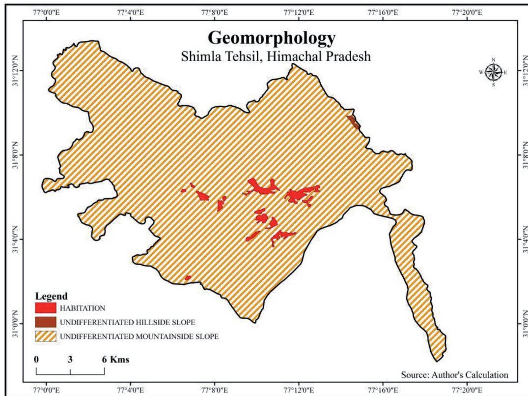
Figure 6. Geomorphology.
