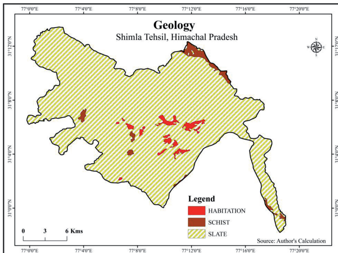
Figure 7. Geology.
