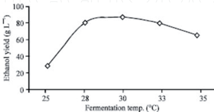
Figure 4. Effect of temperature on bioethanol yield [61].
