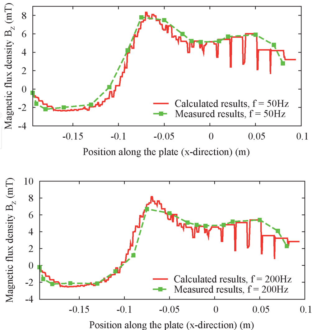
Figure 21. The comparison of the calculated results with the measured results on magnetic flux densities at y = 72\text{ mm} , with \mu_{r,\text{plate}} = 1 , \sigma_{r,\text{plate}} = 35.26 \frac{\text{MS}}{\text{m}} and different frequencies [4].
