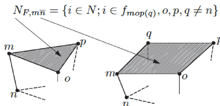
Figure 8. Determination of the facet associated with N_{F,m\bar{n}} [6].
