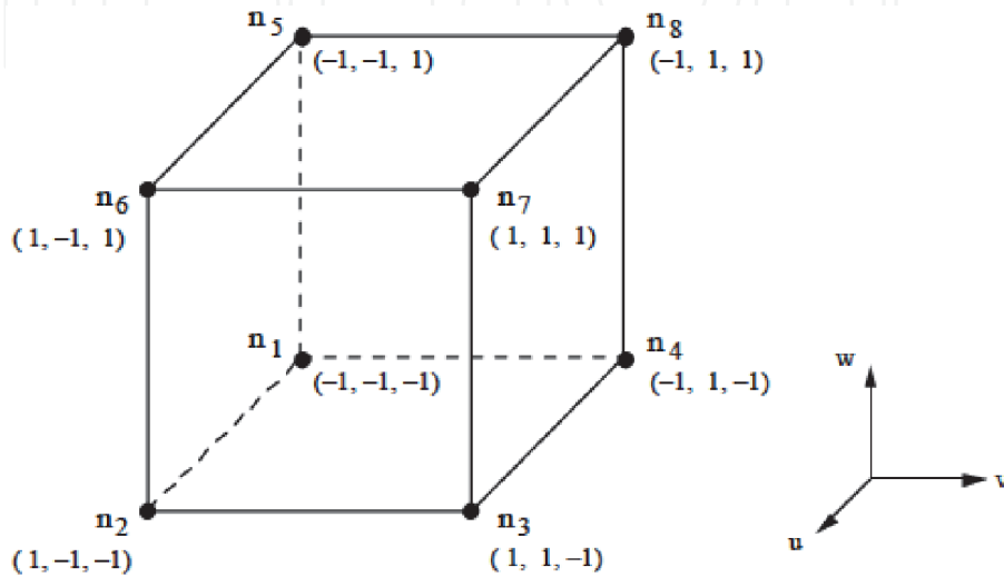
Figure 15. Reference hexahedron of type I [6].
