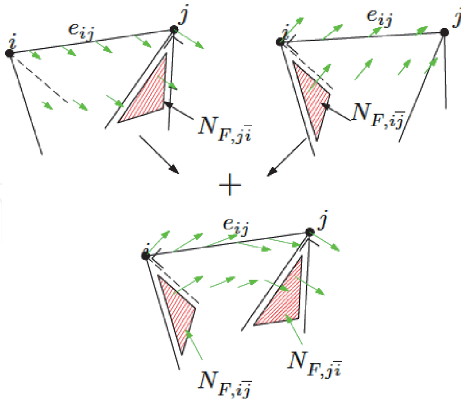
Figure 9. Geometric interpretation of the edge function s_e (35) [6].
