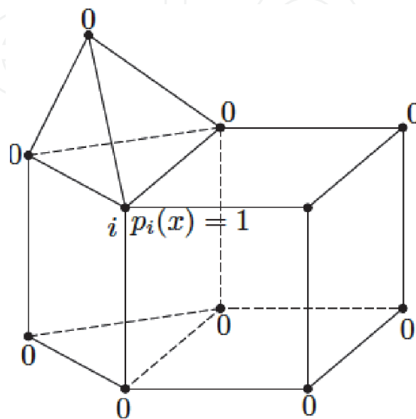
Figure 6. Collection of different geometric elements [6].
