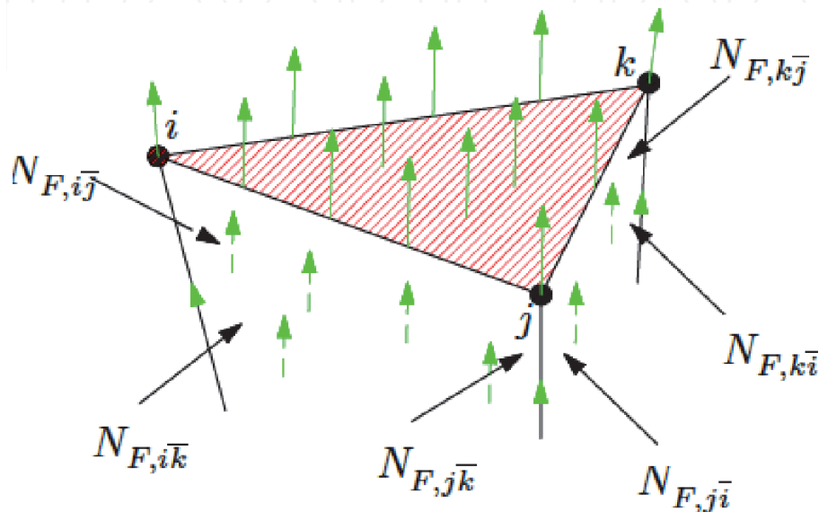
Figure 11. Geometric interpretation of the facet function s_f (36) [6].
