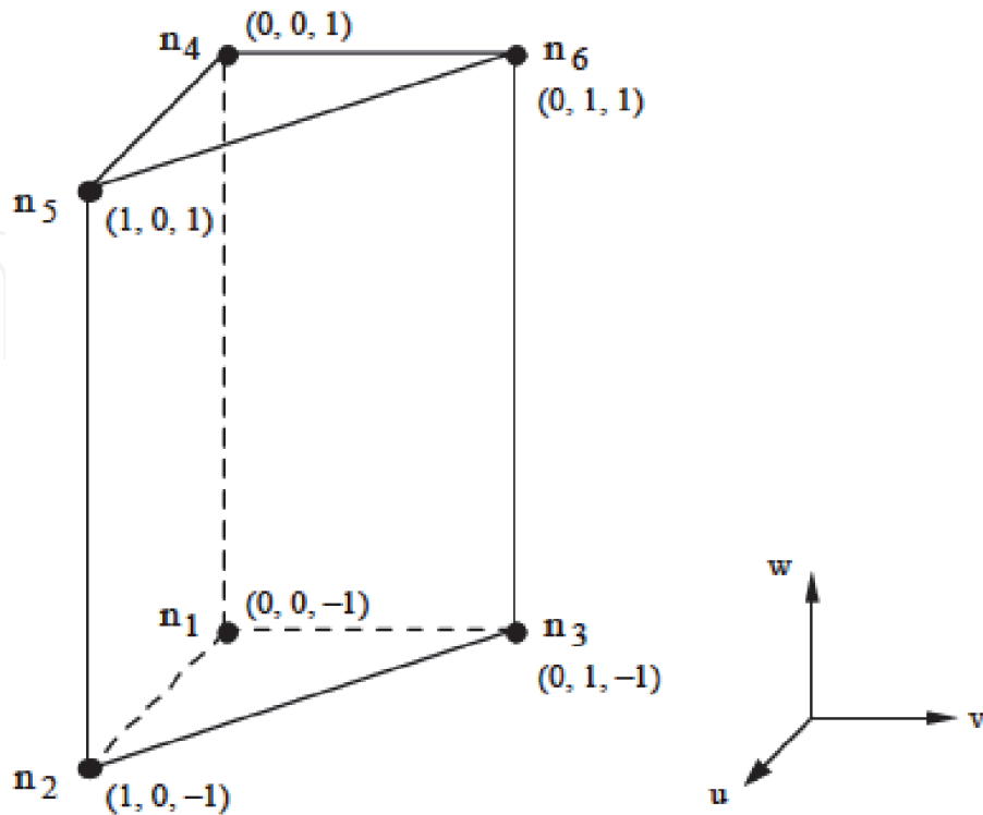
Figure 17. Reference prism of type I [6].
