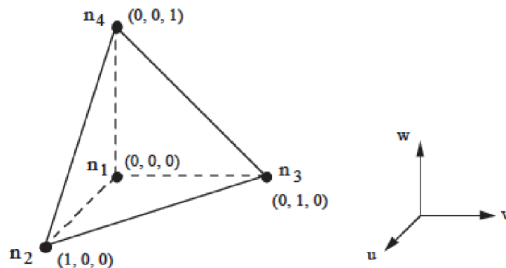
Figure 13. Reference tetrahedron of type I [6].
