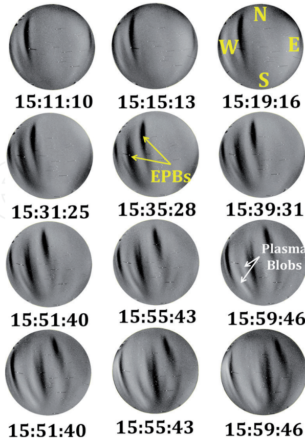
Figure 1. Sequences of images of OI 630.0 nm obtained on 17-18 January, 2012 in IST at Kolhapur. Yellow and white arrows are showing dark and bright (EPB and plasma blob) respective structures in images.
