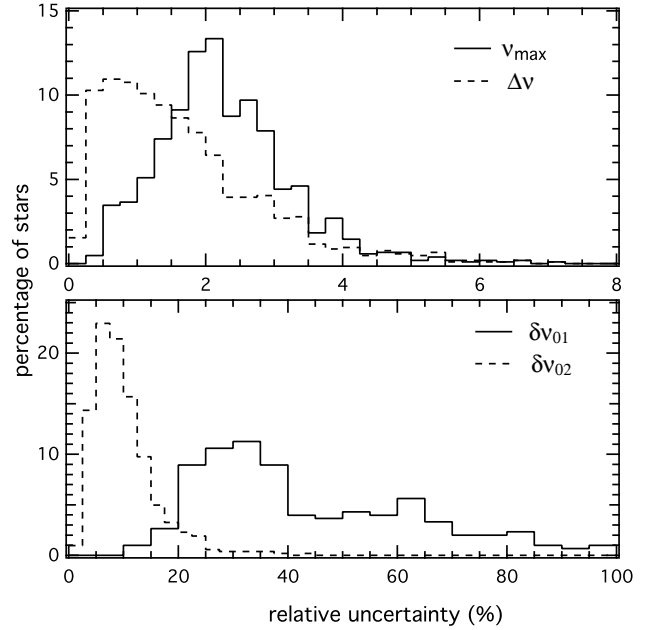
Fig. 4. Histograms of the relative uncertainties for v_{\max} , the large frequency separation \Delta\nu , and the small separations \delta\nu_{01} and \delta\nu_{02} .
