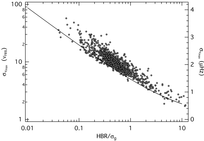
Fig. 3. The uncertainty in v_{\max} in actual value (right axis) and in units of the frequency resolution as a function of the ratio between the height-to-background ratio (HBR) and the width of the power excess, \sigma_g . The line indicates a power-law model for the lower envelope.
