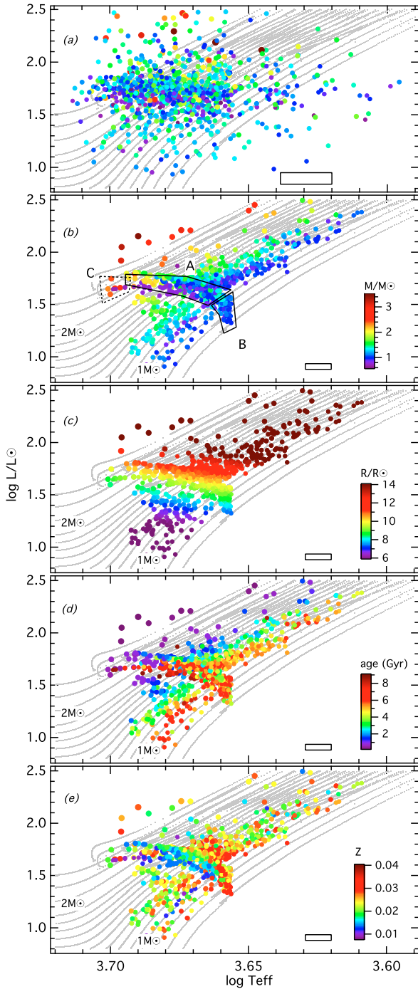
Fig. 9. H-R diagram showing the location of our red-giant sample as directly determined from Eqs. (4) and (5) using the KIC effective temperatures (panel a ) and from the comparison with the stellar model grid (panel b ) to e ). The colour code (in the online version only) indicates the stellar mass ( a and b ), radius c ), age d ), and metallicity ( e ), where the radius scale has been truncated below 6 and above 14 R_{\odot} . Grey lines show solar-metallicity BaSTI evolutionary tracks. The boxes given in the lower right corners illustrate typical uncertainties.
