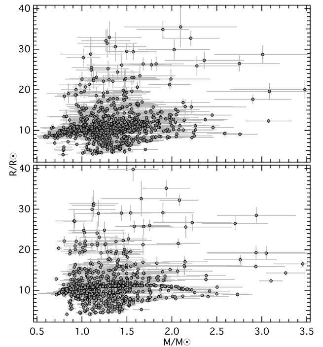
Fig. 8. The stellar radius as a function of mass for the sample of red giants as directly determined from Eqs. (4) and (5) using the KIC effective temperatures (top) and from the comparison with the stellar model grid (bottom).
