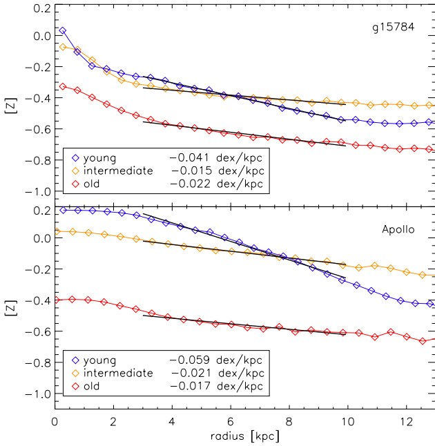
Fig. 1. Stellar radial [Z] gradients, for disk stars in three different stellar populations: young (blue) is defined as stars formed in the last 100 Myr, intermediate (yellow) is defined as stars formed 6 to 7 Gyr ago, and old (red) is defined as stars older than 10 Gyr. Fits to the disk are overdrawn in black; the length of the black line corresponds to the region of the disk used in the fitting (see text for details). For clarity, only two galaxies are shown, one from MUGS (g15784, upper panel) and one from RaDES (Apollo, lower panel).
