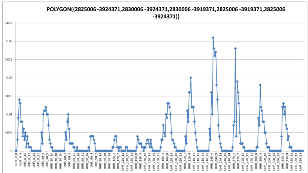
Figure 98: Amherst CWA Histogram Data broken down by 30° sector in side-by-side format
