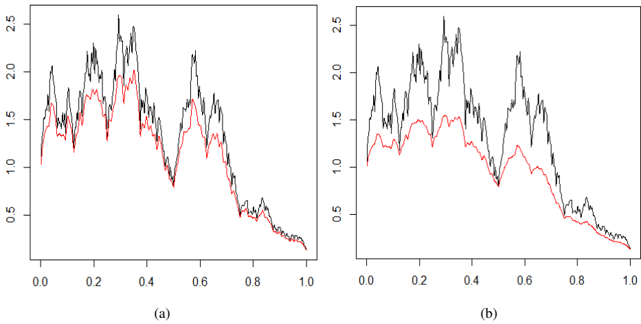
Figure 2. The mis-specification of (a) H = 0.6 and (b) H = 0.8 : graphs of X (black) and X_p (red).
