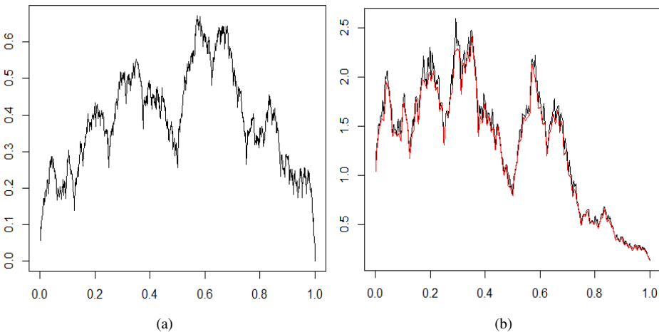
Figure 1. (a) Function g ; (b) solutions X (black) and X_p (red) for H = 0.51 .
