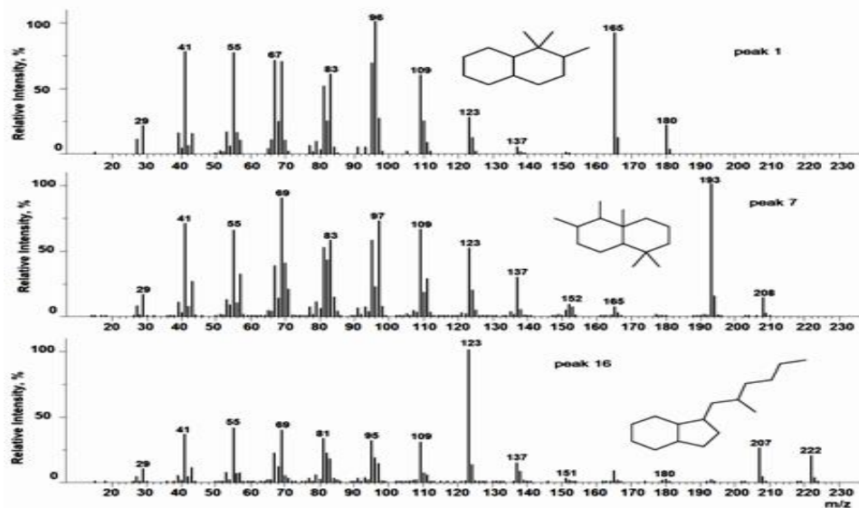
Fig. 7. Mass spectra of (c) 1,1,2-Trimethyldecaline (peak 1), 1,2,3,7,7-Pentamethyldecaline (peak 7) and 1-(2-Methylhexyl)perhydroindane (peak 16).
