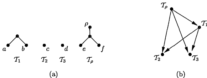
FIGURE 3. (a) A maximum-acyclic-agreement forest \mathcal{F} for \mathcal{T} and \mathcal{T}' in Fig. 2 and (b) the graph G_{\mathcal{F}} .
