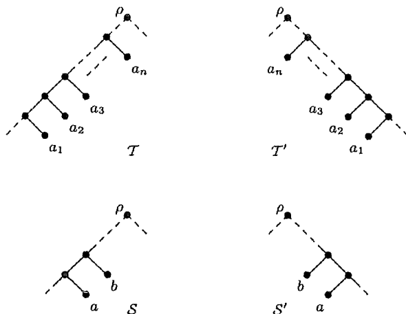
FIGURE 5. Two weighted phylogenetic trees reduced under Rule 2, where S and S' are the resulting trees.
