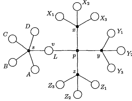
FIGURE 4. The 3-tree T_1 .
