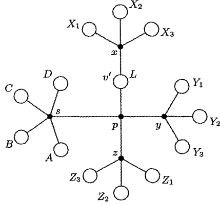
FIGURE 5. The 3-tree T_2 .
