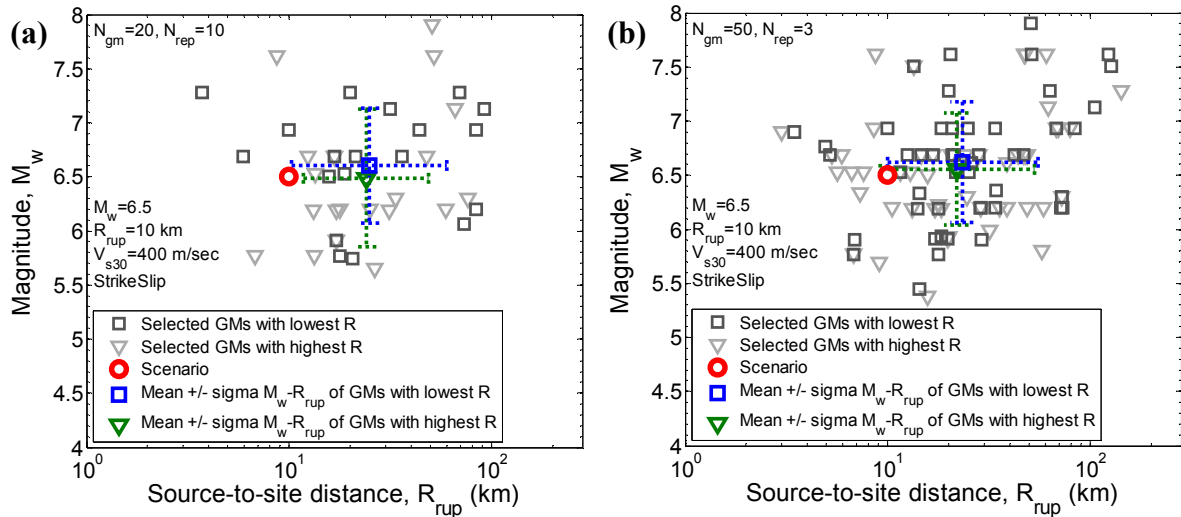
Figure 20: M_w - R_{rup} distribution of selected motions for the M6.5R10V400 rupture scenario using weight vector case 6 (i.e., SA, AI, CAV, D_{s575} , D_{s595} ): (a) 20; and (b) 50 motions
