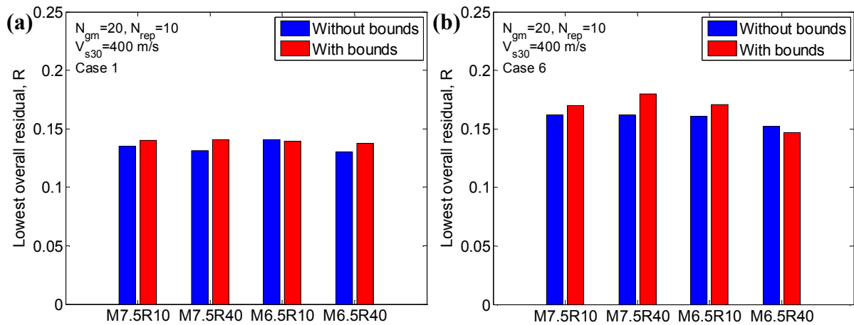
Figure 25: Overall residual (i.e., R value) of selected ensemble of 20 motions with and without bounds on the implicit causal parameters for all the rupture scenarios with V_{s30}=400 m/s site condition, using weight vector: (a) case 1 (i.e., SA only); (b) case 6 (i.e., SA, AI, CAV, D_{s595} , and D_{s575} )
