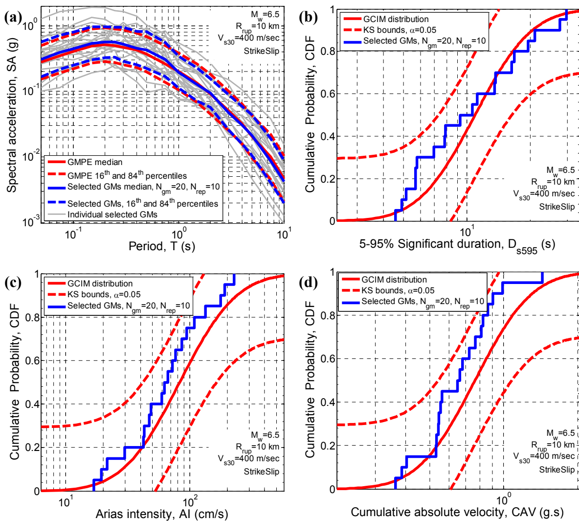
Figure 24: Properties of selected motions after applying bounds on casual parameters using weight vector case 6 (i.e., SA, AI, CAV, D_{s595} , and D_{s575} ) for the M6.5R10V400 rupture scenario: (a) SA ordinates; cumulative distribution of (b) D_{s595} ; (c) AI; and (d) CAV
