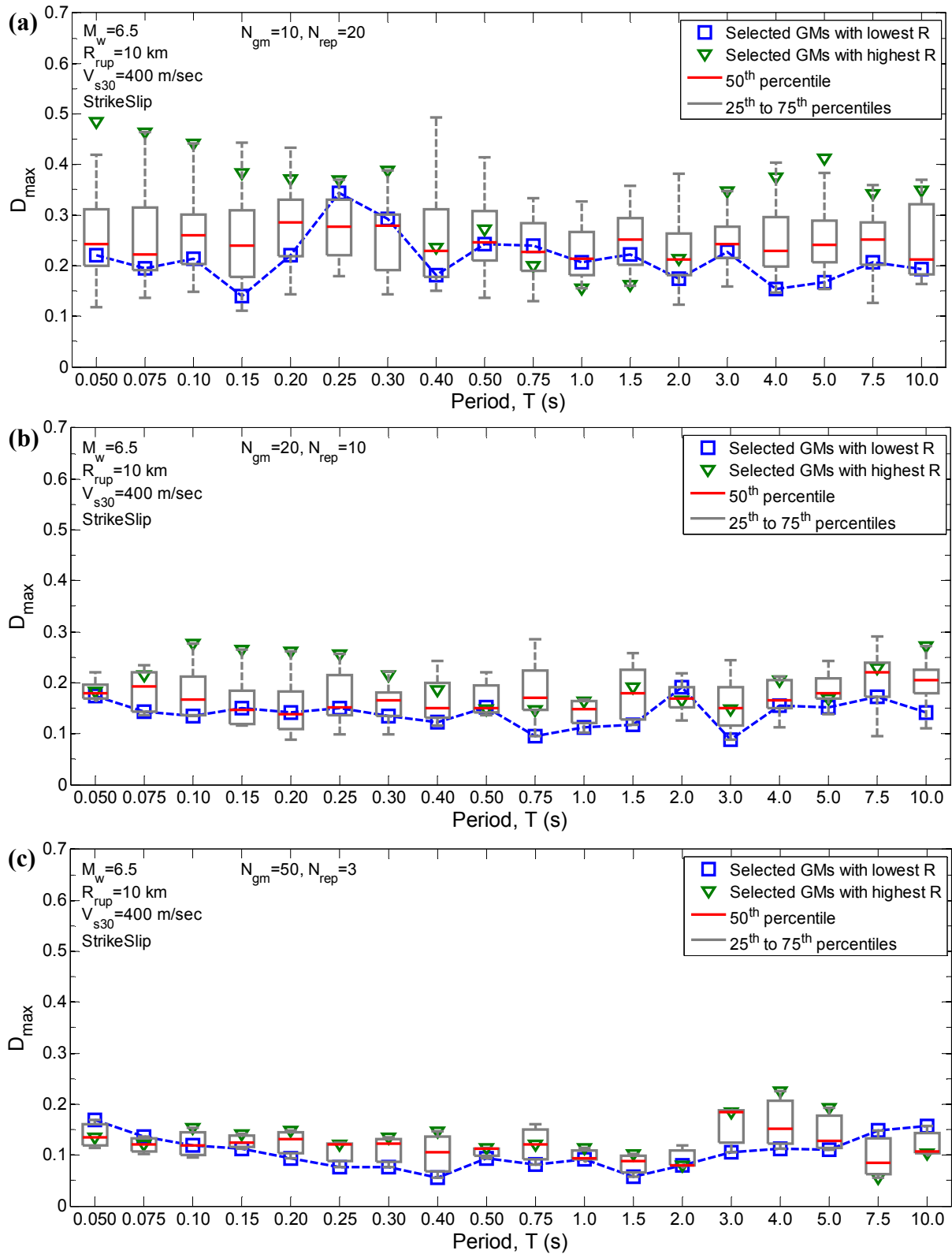
Figure 16: D_{max} value of SA ordinates of selected motions using weight vector case 1 (i.e., SA only) for the M6.5R10V400 rupture scenario with: (a) N_{gm} = 10 ; (b) N_{gm} = 20 ; (c) N_{gm} = 50 ;
