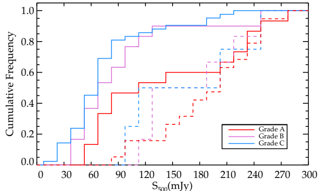
Figure 2. Cumulative frequency distribution of S_{500} flux densities for the near-IR subset of SMG candidate lensing systems. The solid red, purple, and blue lines represent Grade A, B, and C sources respectively. For comparison, the dashed lines are from the sub-mm sample from Bussmann et al. (2013), converted to the same near-IR grading scheme. Grade A sources tend to have smaller cumulative fractions than Grade B and C sources with increasing values of S_{500} , which supports the idea that 500 \mu\text{m} -bright sources have a higher probability of being lensed.
