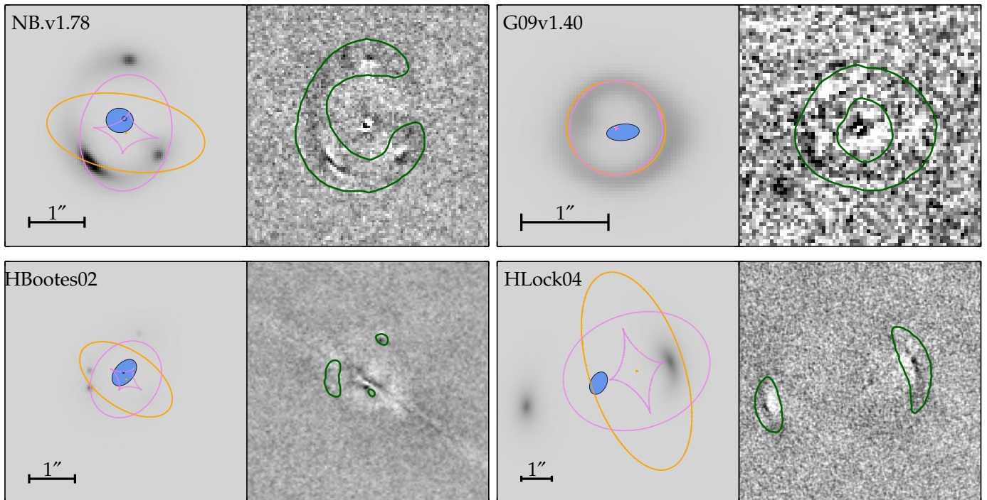
Figure 10. Lens models of the lens Grade A subsample that overlaps with Bussmann et al. (2013), with the foreground lens parameters fixed to sub-mm derived values. The images are displayed at the same scale as their Fig. 4 counterparts. North is up and east is left for all the panels.
