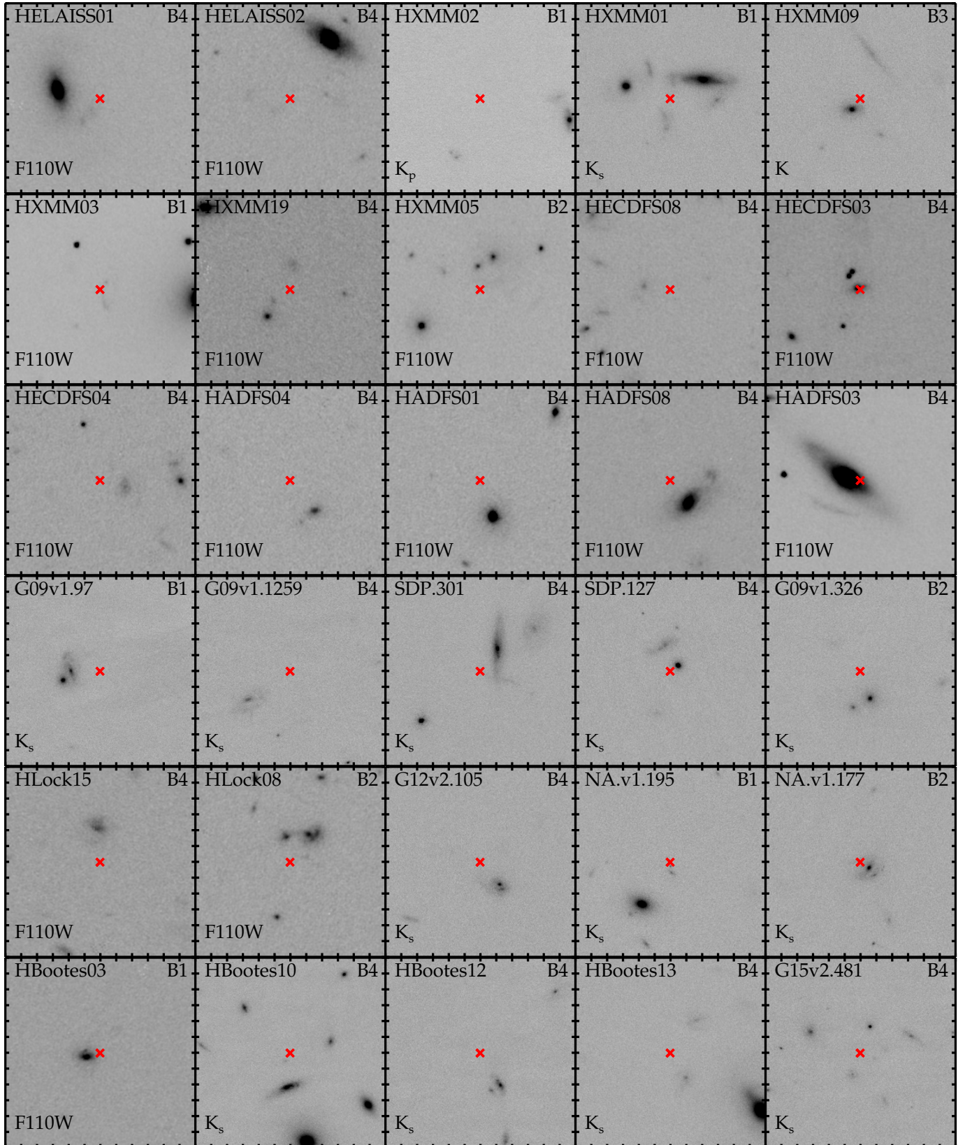
Figure 11. Near-IR images of Grade B sources, oriented north is up and east is left for all images. Each tick mark is 1'' and the size of each panel is 12'' . The near-IR band and the complete lens grade are shown in the lower left and upper right corners, respectively. The red crosses represent the measured Herschel position.
