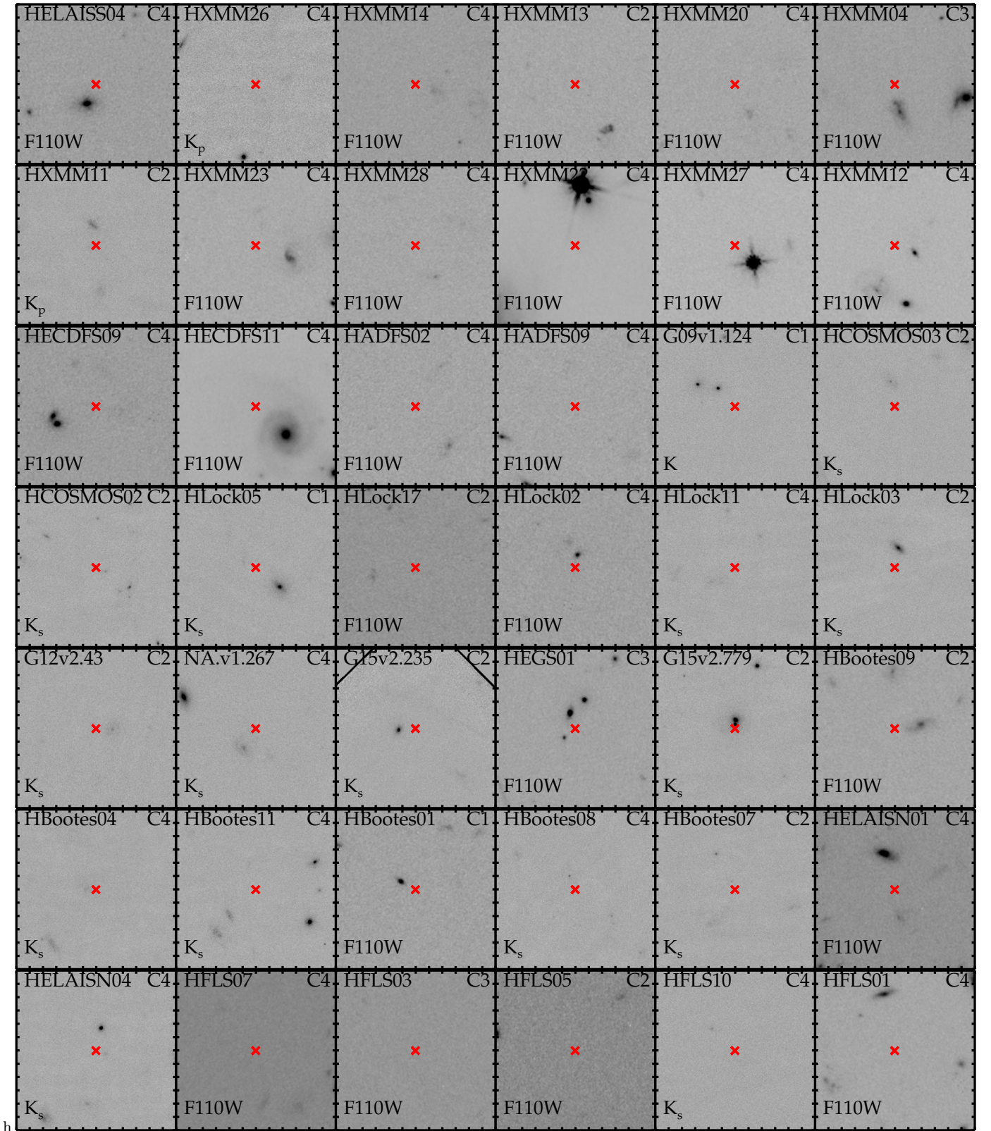
Figure 12. Near-IR images of Grade C sources, oriented north is up and east is left for all images. Each tick mark is 1'' and the size of each panel is 12'' . The near-IR band and the complete lens grade are shown in the lower left and upper right corners, respectively. The red crosses represent the measured Herschel position.
