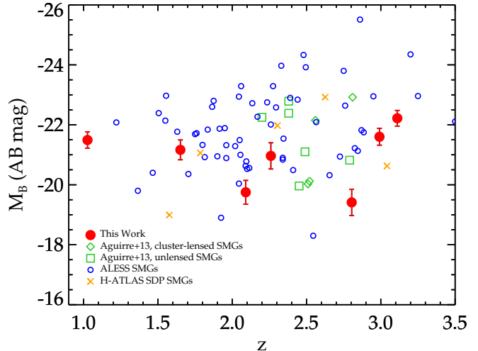
Figure 8. Rest-frame magnification-corrected absolute B -band magnitudes ( M_B ) for Grade A1 and A2 candidates versus redshift. Open diamonds and squares represent cluster-lensed and unlensed SMGs from Aguirre et al. (2013), respectively. Open circles are unlensed ALESS SMGs from Simpson et al. (2013). The M_B values for lensed SMGs are consistent with unlensed SMGs at z > 1 , but tend to lie towards the fainter end of the distribution.
