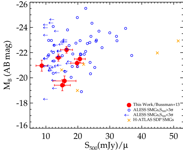
Figure 9. Rest-frame magnification-corrected absolute B -band magnitudes ( M_B ) for Grade A1 and A2 candidates versus magnification corrected SPIRE S_{500} . We use the sub-mm magnification from Bussmann et al. (2013) when available to correct for the observed S_{500} . Open circles are unlensed ALESS SMGs from Swinbank et al. (2014) and Simpson et al. (2013). Our sample of lensed SMGs have consistent S_{500} values for a given M_B relative to the unlensed population, suggesting that Herschel -selected lensed SMGs are similar to classical unlensed 850\ \mu\text{m} -bright SMGs.
