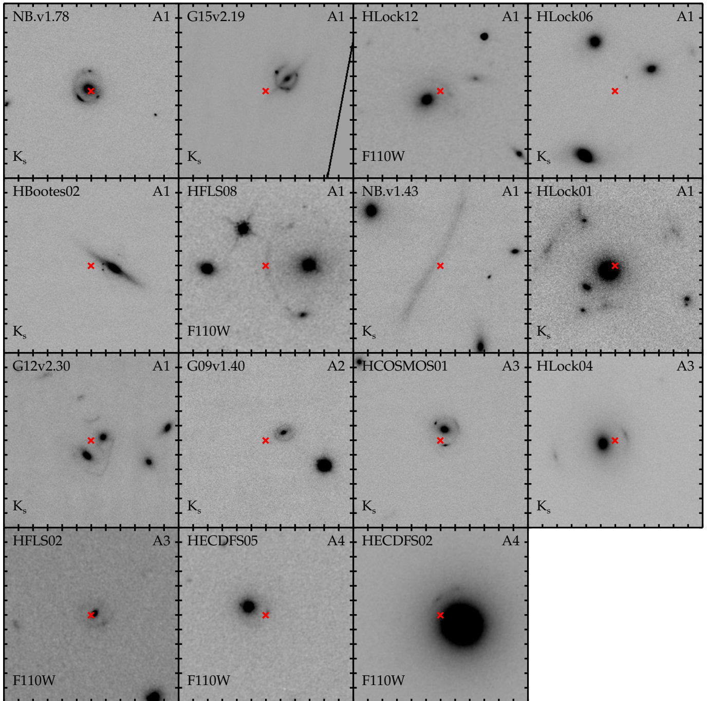
Figure 3. 12'' cutouts of all lens Grade A lensed SMGs, with each tick mark corresponding to 1'' and oriented with north is up and east is left. All have either been observed using Keck NIRC2-LGS-AO K_s or HST /WFC3 F110W. The red cross marks the measured Herschel position. Contrast levels are varied in each image to highlight the observed lensing morphology.
