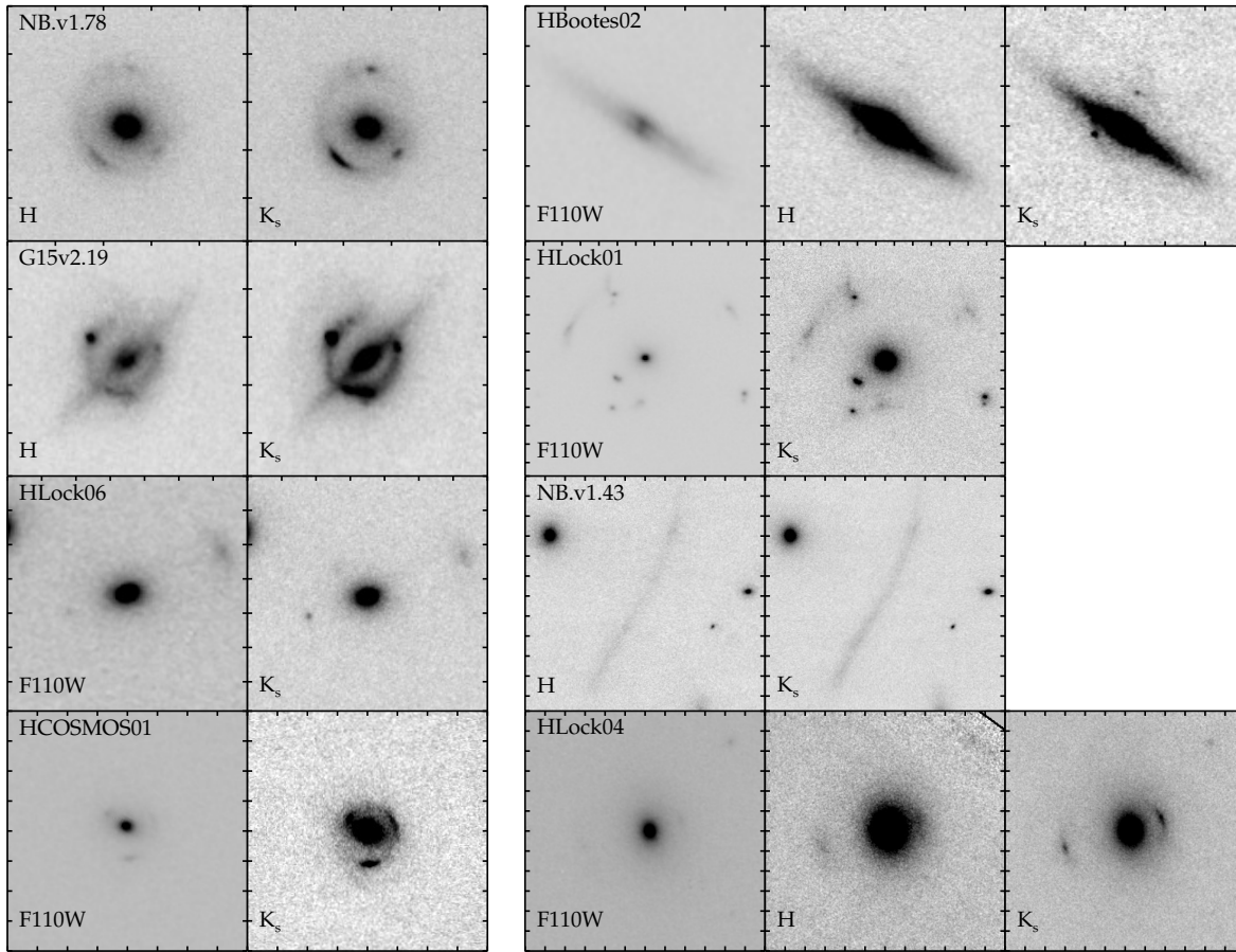
Figure 13. Multi-wavelength high-resolution near-IR for Grade A lensed SMGs, oriented north is up, east is left for all images. The near-IR band is labeled on the lower left corner. Each tick mark represents 1'' . All images are scaled to have consistent brightness units.
