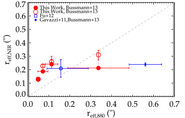
Figure 6. Intrinsic effective radii of lensed SMGs in the near-IR compared with 880 \mu\text{m} . Filled symbols are from independent analyses in the near-IR and sub-mm. Open symbols denote consistent foreground lens parameters between the near-IR and sub-mm. Here, the foreground lens parameters are fixed to those derived from the sub-mm (Bussmann et al. 2013). Most of the SMGs lie above the line of one-to-one correspondence (dashed line), showing that their dust emission is typically less extended than the rest-frame optical (likely stellar) emission. This is consistent with the observed differential magnification (Fig. 5), and suggests that smaller emission regions are generally more highly magnified.
