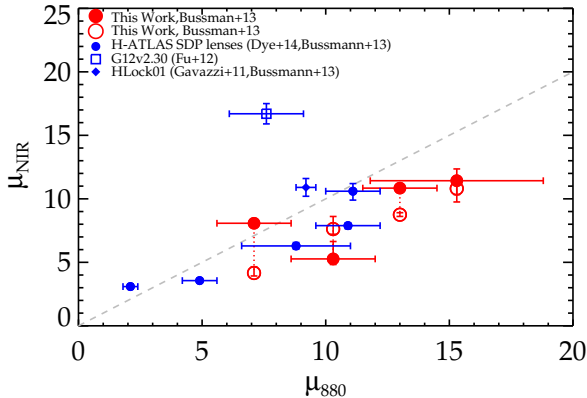
Figure 5. \mu_{\text{NIR}} vs \mu_{880} . Filled symbols are magnification values from independent near-IR and sub-mm lensing analyses. Open symbols denote best-fit lens models using consistent foreground lens parameters in the near-IR and sub-mm. For our work, we fix sub-mm lens parameters from Bussmann et al. (2013) to our near-IR data. The blue circles, diamonds and square are near-IR data points from Dye et al. (2014); Gavazzi et al. (2011), and Fu et al. (2012), respectively, with the corresponding sub-mm magnifications from Bussmann et al. (2013), if available. The dashed line shows one-to-one correspondence between \mu_{\text{NIR}} and \mu_{880} . Most sources lie below this line, with \mu_{\text{NIR}} < \mu_{880} . Differential magnification is observed and is likely due to spatial variations or a morphological difference between the near-IR (stellar) and sub-mm (dust) emission.
