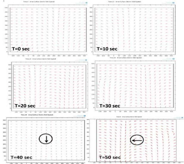
FIGURE 9: Shows normalized arrow plots. At the center of the chamber rotational arrows are marked for clarity.
