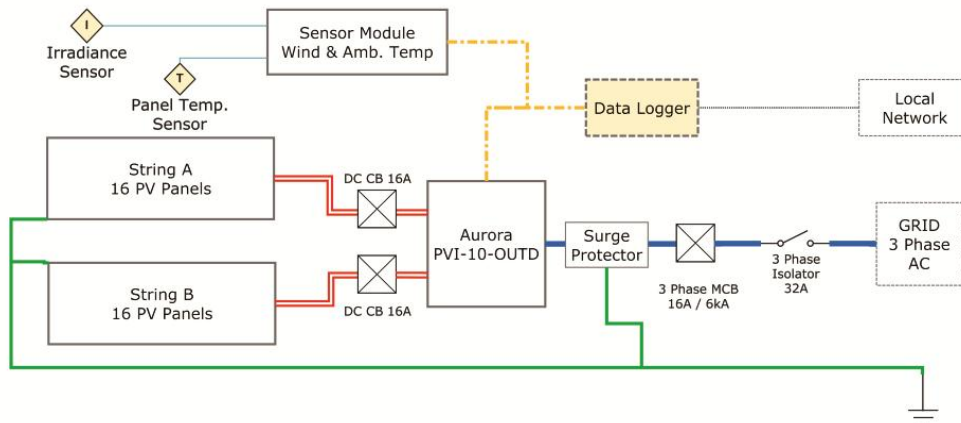
FIGURE 2: DESIGN A SCHEMATIC INSTALLED IN TAKUILAU COLLEGE & BEULAH COLLEGE.
