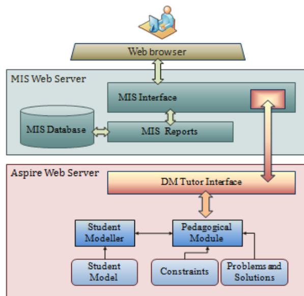
Figure 1. Architecture of DM-Tutor embedded with the MIS
