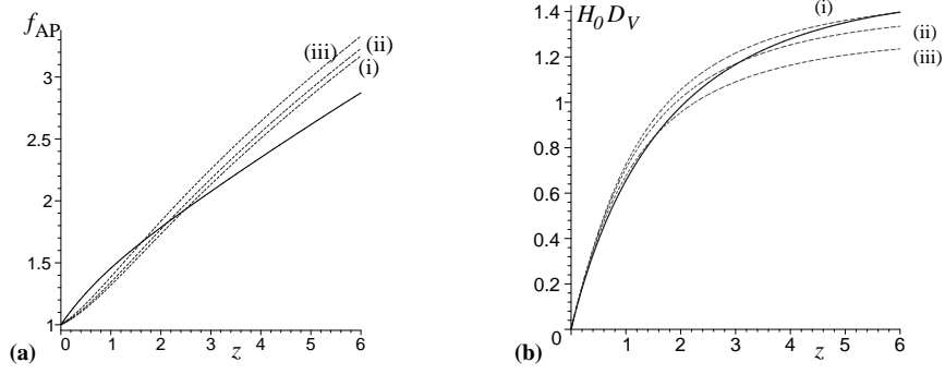
FIGURE 5. (a) The Alcock–Paczyński test function f_{\text{AP}} = HD/z ; and (b) the BAO radial test function H_0 D_V = H_0 D f_{\text{AP}}^{-1/3} . In each case the timescape model with f_{v0} = 0.762 (solid line) is compared to three spatially flat \Lambda CDM models with the same values of (\Omega_{M0}, \Omega_{\Lambda0}) as in Fig. 1 (dashed lines).
