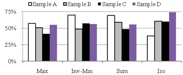
Figure 11. Estimation rate of NP training set
