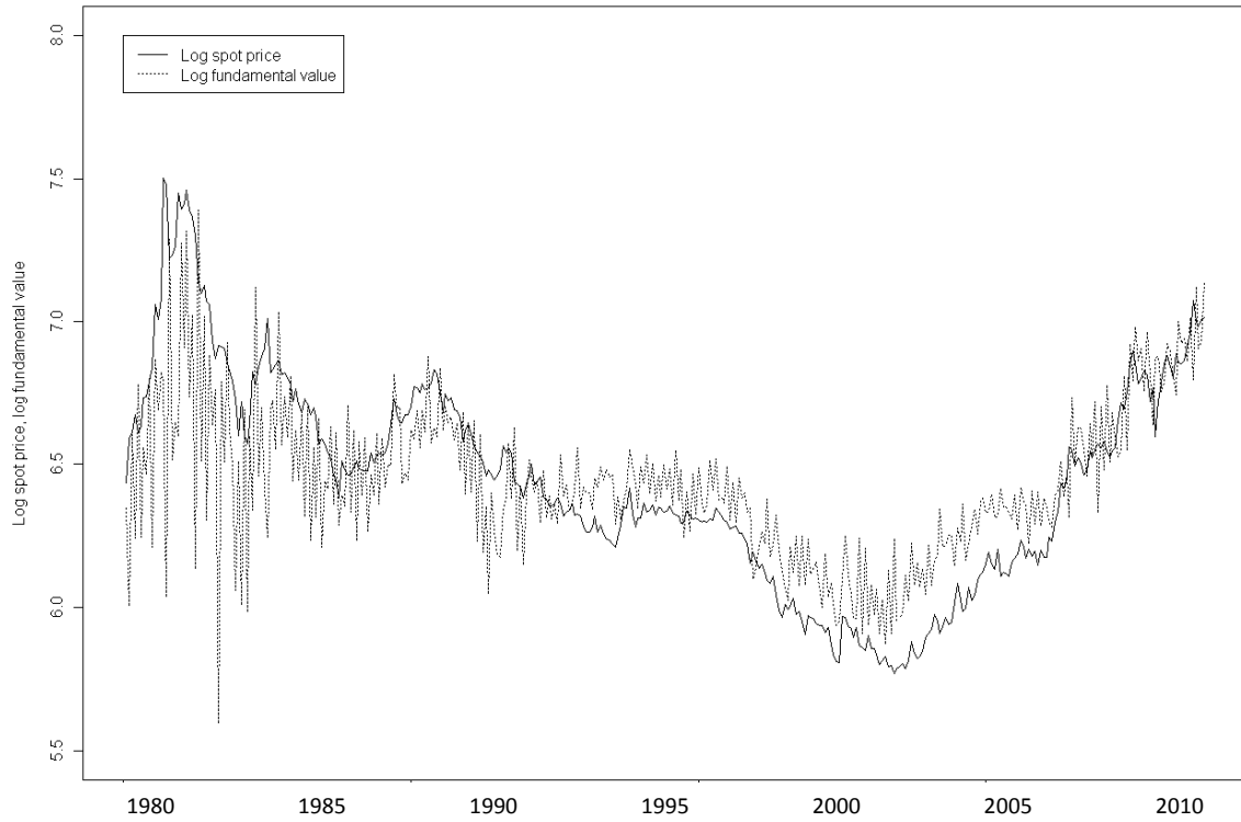
Figure 5: Real spot price and fundamental value (in logs)
