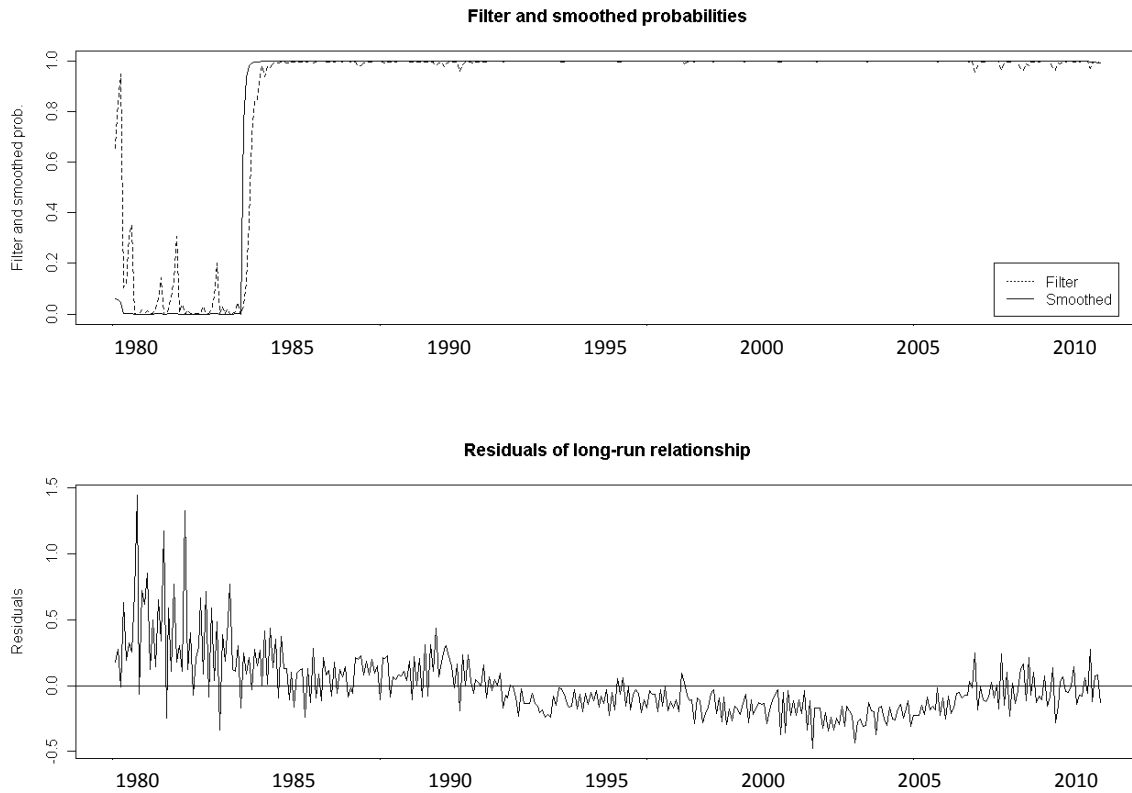
Figure 7: Filter and smoothed probabilities, and residuals of the long-run relationship (based on real data)
