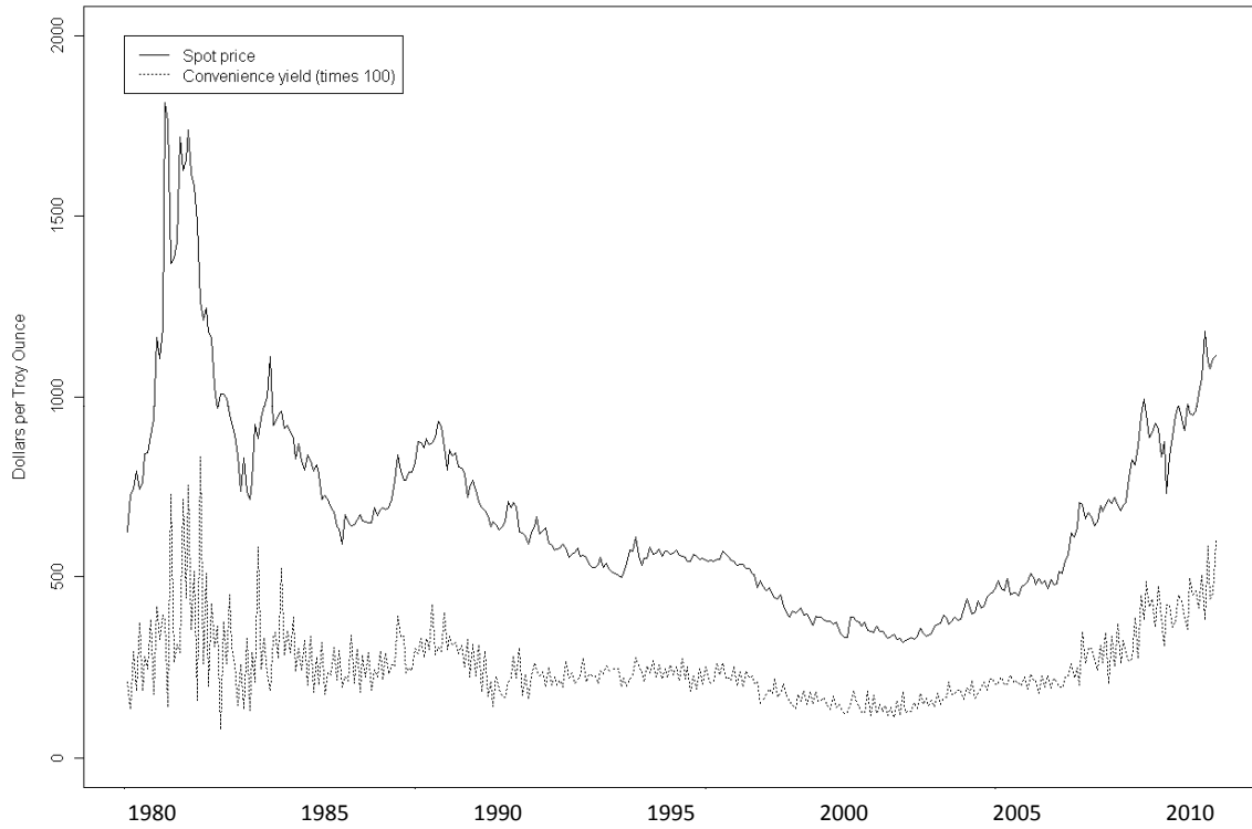
Figure 2: Real spot price and convenience yield
