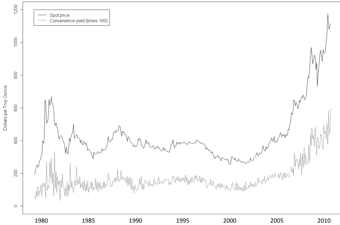
Figure 1: Nominal spot price and convenience yield
