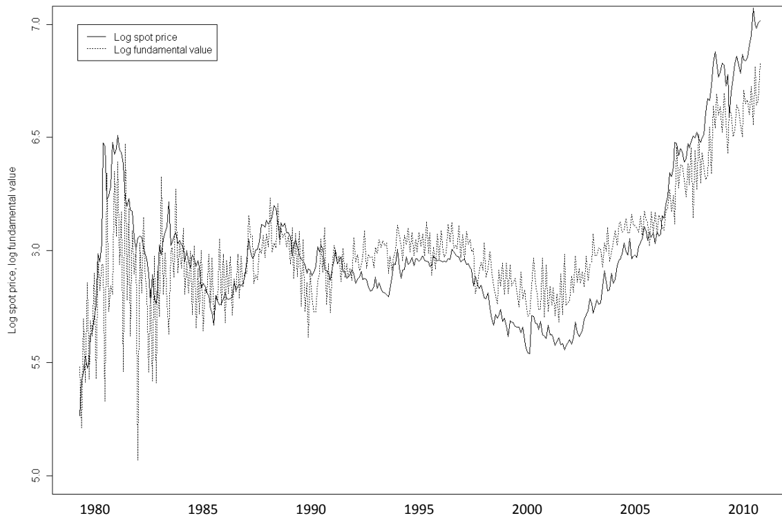
Figure 4: Nominal spot price and fundamental value (in logs)
