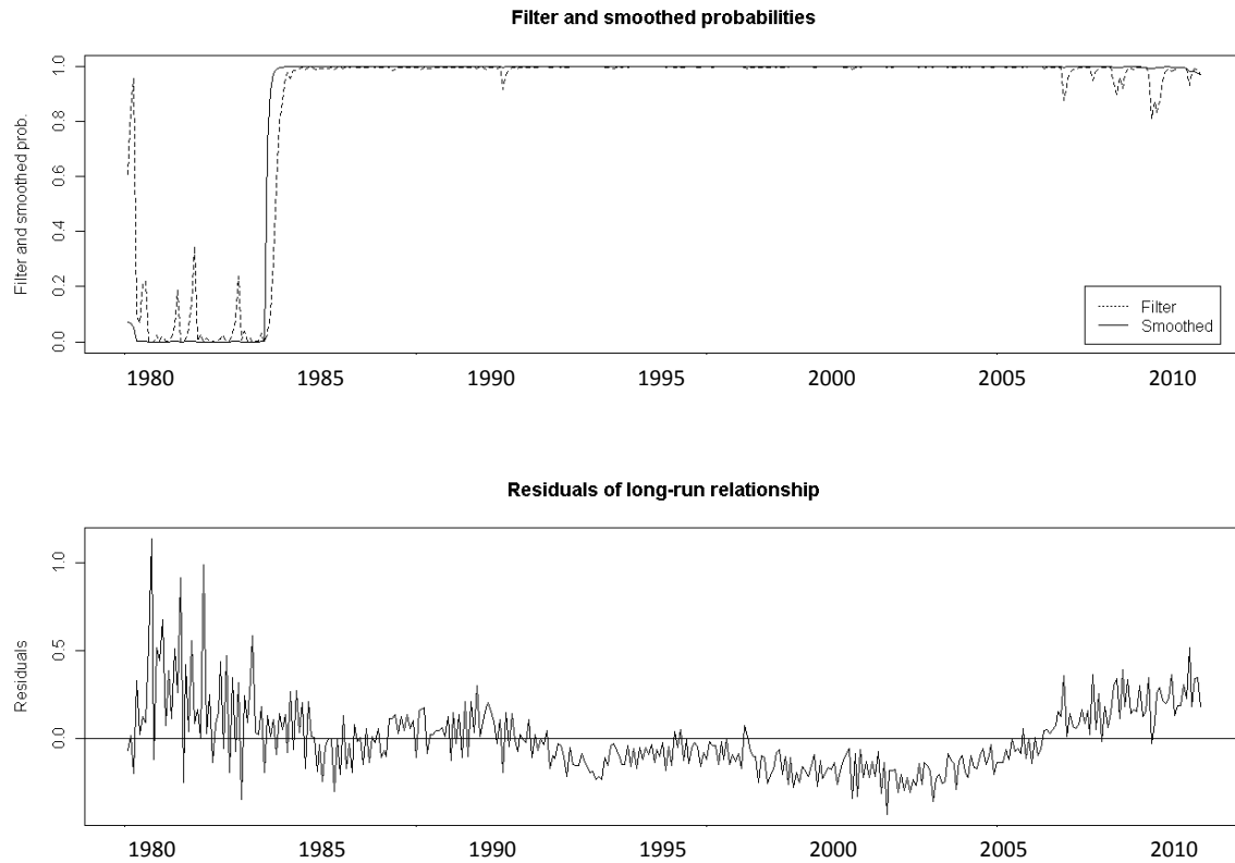
Figure 6: Filter and smoothed probabilities, and residuals of the long-run relationship (based on nominal data)
