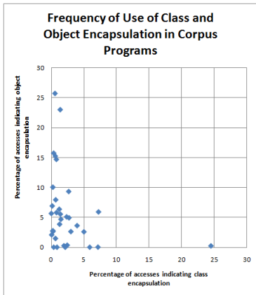
Figure 7: Corpus use of object and class encapsulation.
