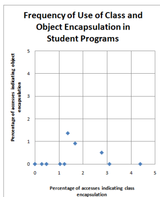
Figure 8: Student use of object and class encapsulation.
