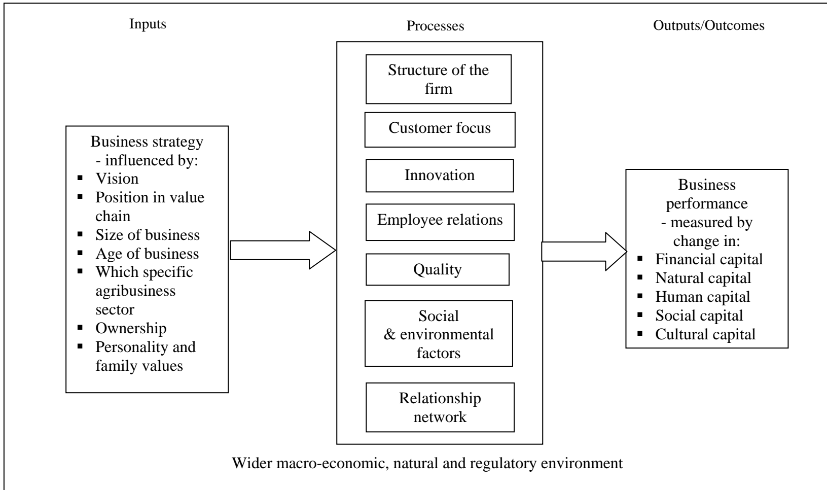
Figure 5.1: Proposed model
