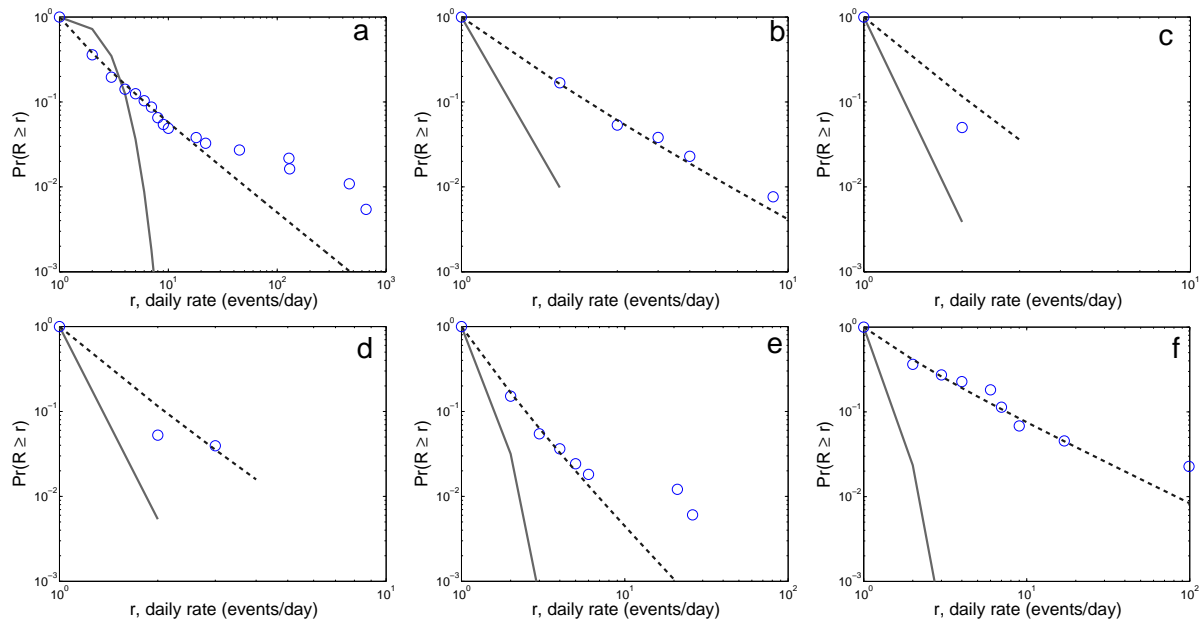
Figure 3.7: Cumulative Distribution Function (CDF) of landslide daily rates (blue circles); best Kolmogorov-Smirnov power-law fit (black dashed line). a) New Zealand landslides; b) Yosemite landslides; c) Grenoble cliffs landslides; d) Val d'Arly cliff landslides; e) Australia landslides; f) Wollongong landslides. The grey line represents the Poisson function which fits best the values. Values of exponent b and lower cutoffs are given in Table 3.6. Note that i) the fit is slightly curved for daily rates lower than 6 events/day, which is inherent in the definition of a discrete power-law (e.g. Clauset et al., 2009) and ii) the exponent of the CDF B is equal to b - 1 (e.g. Bonnet et al., 2001).
