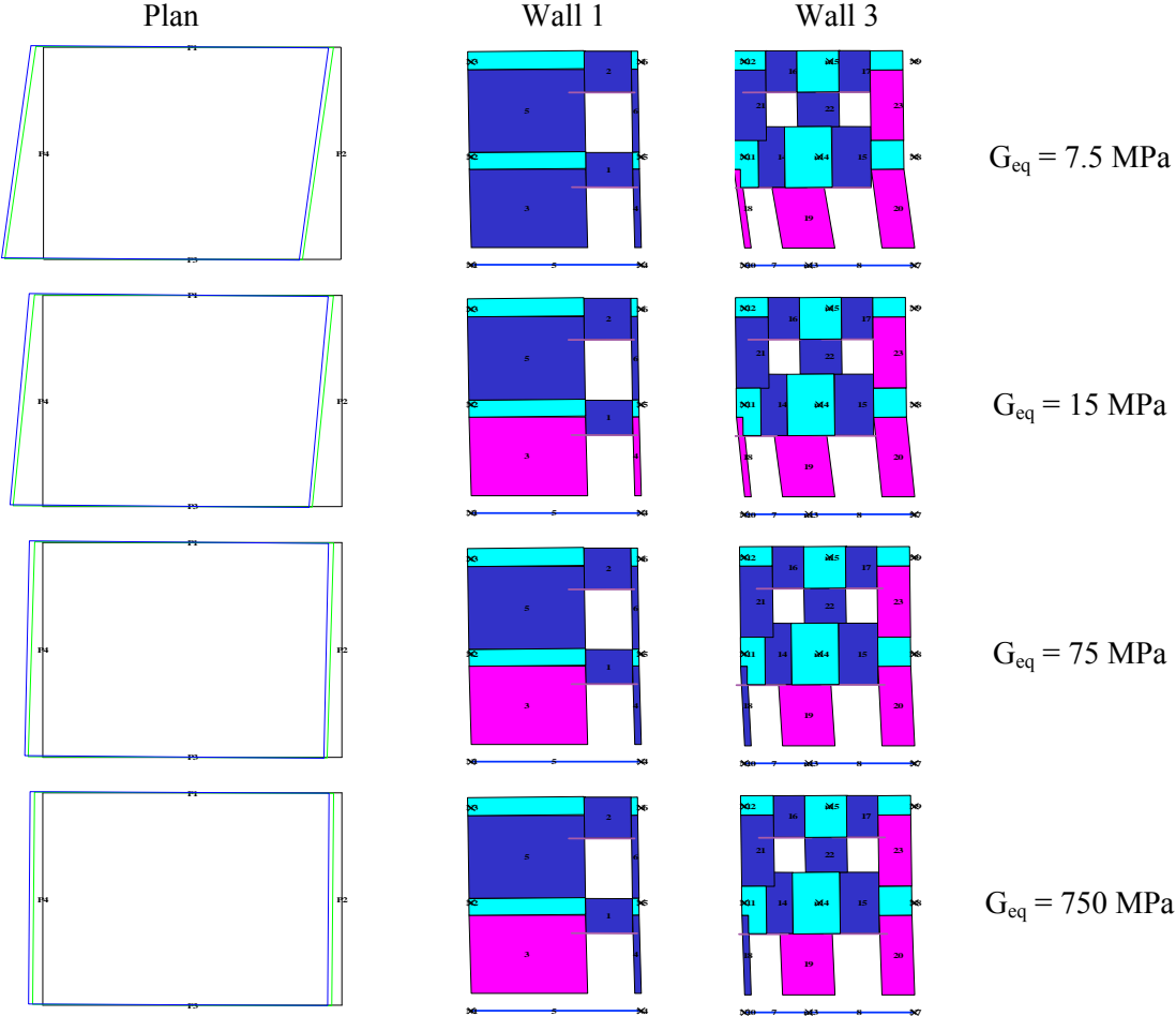
Figure 10. Deformed shape for different diaphragm stiffness.
