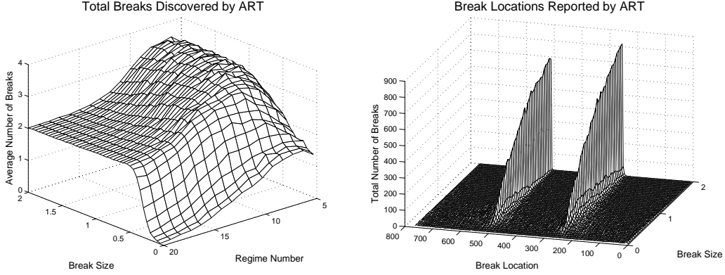
Figure 3: Left panel: Total number of breaks reported by ART in the two offsetting break simulations with BIC pruning. Right panel: The locations of the breaks reported for the series with regime length 256 data points, i.e. regime 16 in the left panel. The series had Gaussian noise.
