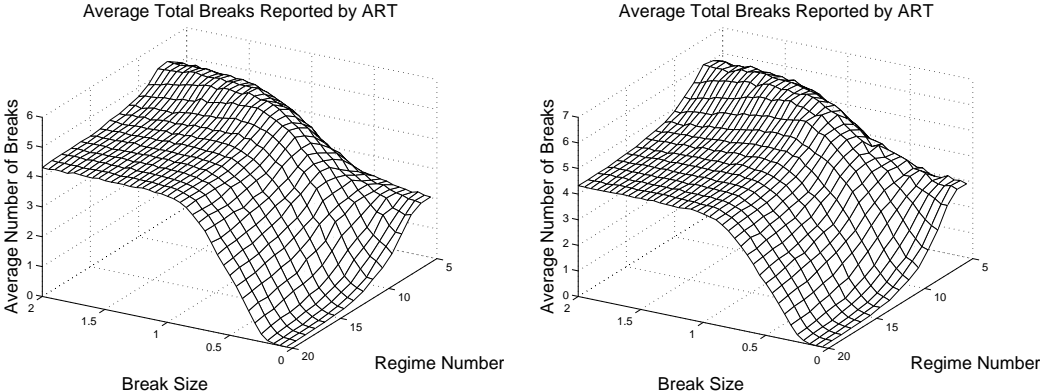
Figure 5: The average total number of breaks reported by ART when using BIC pruning for the noisy square wave with gamma distributed noise (left panel) and geometrically distributed noise (right panel). The series had four breaks.
