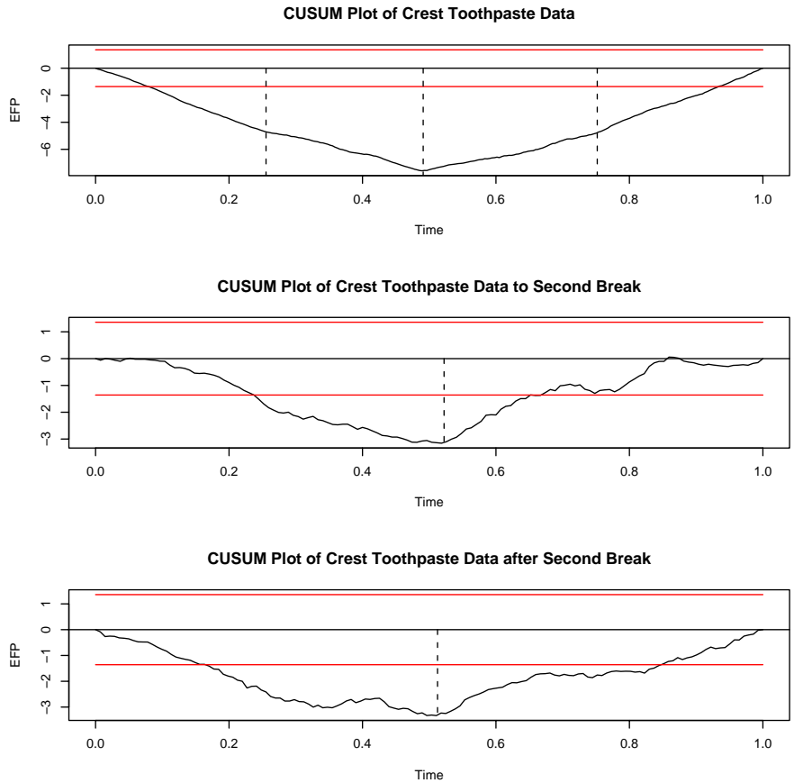
Figure 14: The top panel is the CUSUM plot for whole series. The middle panel is the CUSUM plot to the break in early August 1960. The bottom panel is the CUSUM plot from the break in August 1960 to the end of the series. The dashed lines are the ART break points. The thin lines about the heavier zero line are the 5% significance level.
